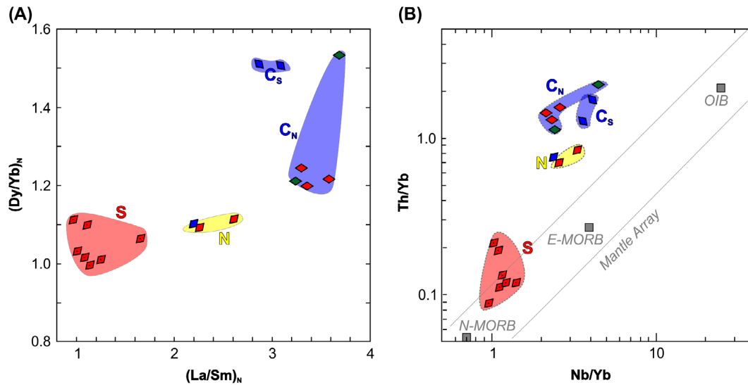
Fig. 6. A. Chondrite-normalised (\text{Dy}/\text{Yb})_N against (\text{La}/\text{Sm})_N , and B. \text{Th}/\text{Yb} against \text{Nb}/\text{Yb} for ca. 2.70–2.66 Ga dykes across the eastern Kaapvaal Craton. The Mantle Array and modelled variable influence of a so-called subduction zone component in B is copied from Pearce (2008). Symbols and colour coding as in Fig. 4.
