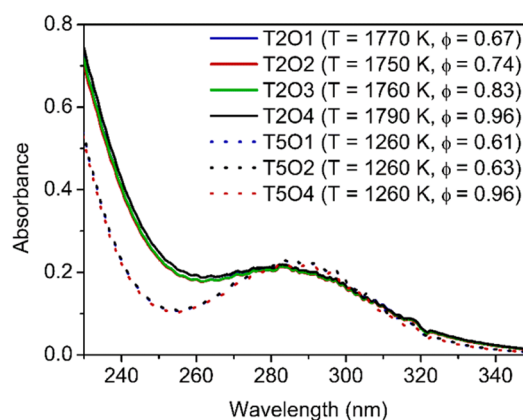
Figure 3. Absorbance of SO 2 with a constant number density in the hot flue gas provided by different lean flames at around 1750 K (T2O1–T2O4) and around 1260 K (T5O1–T5O4).
