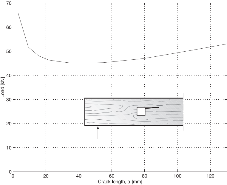
Figure 7.16: Load-bearing capacity of a beam with an internal quadratic hole, h = 600mm .
