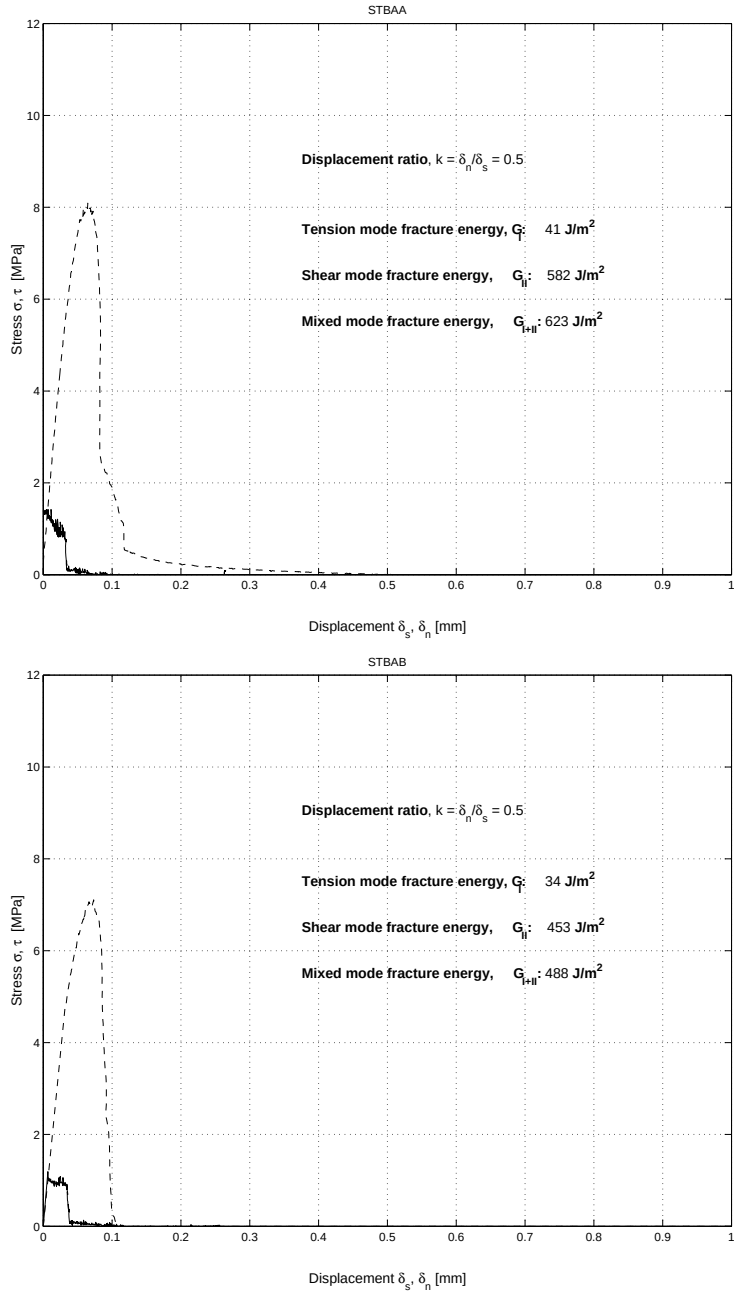
Figure B.4: Stress-displacement diagrams. Displacement ratio k = \frac{\delta_n}{\delta_s} = 0.5
