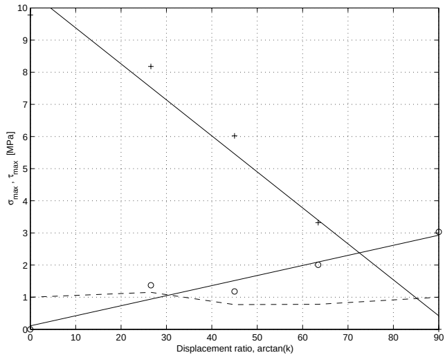
Figure 4.14: Strength versus displacement ratio.
