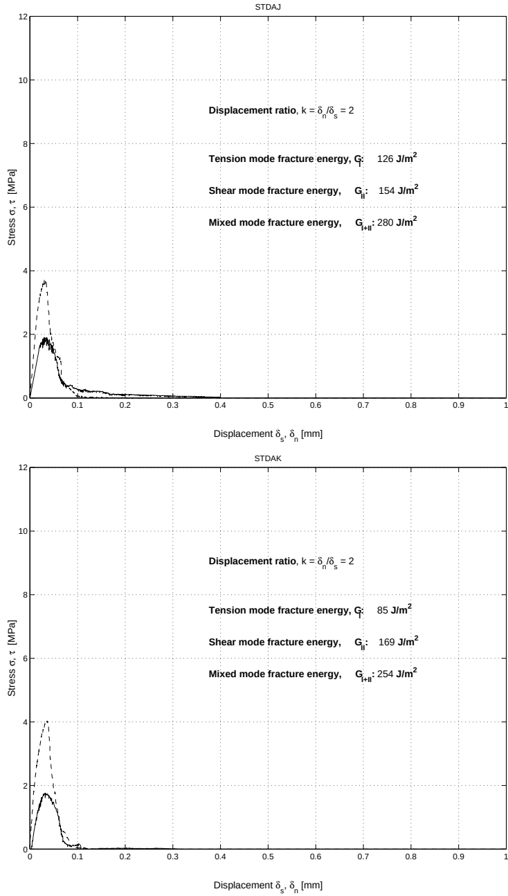
Figure B.14: Stress-displacement diagrams. Displacement ratio k = \frac{\delta_n}{\delta_s} = 2.0
