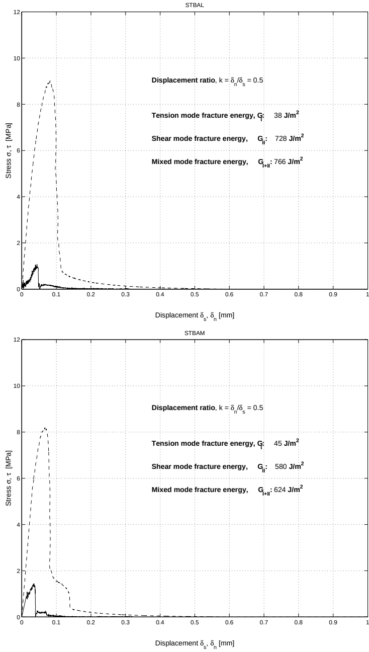
Figure B.8: Stress-displacement diagrams. Displacement ratio k = \frac{\delta_n}{\delta_s} = 0.5
