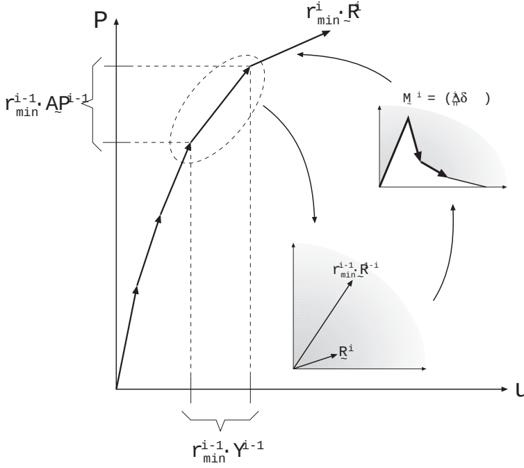
Figure 6.5: Path control
