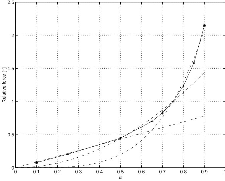
Figure 8.1: End-notched beam. Approximation of load-bearing capacity
