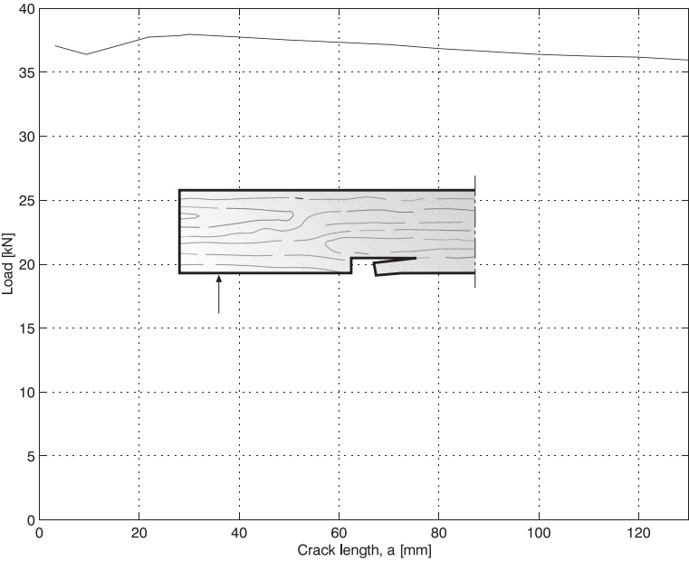
Figure 7.15: Load-bearing capacity of an edge-notched beam, h = 600mm .
