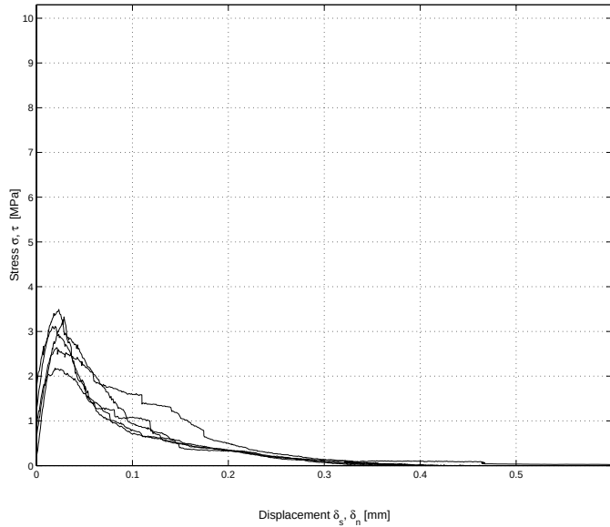
Figure 4.13: Stress-displacement, combined results for k = \infty
