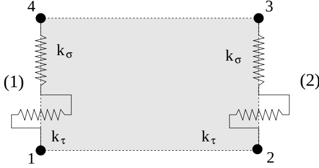
Figure 6.2: Two-spring model
