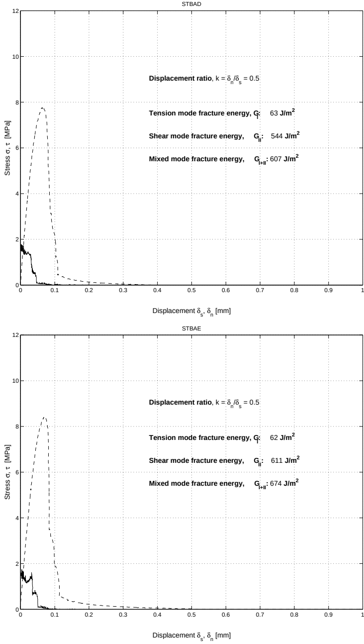
Figure B.5: Stress-displacement diagrams. Displacement ratio k = \frac{\delta_n}{\delta_s} = 0.5
