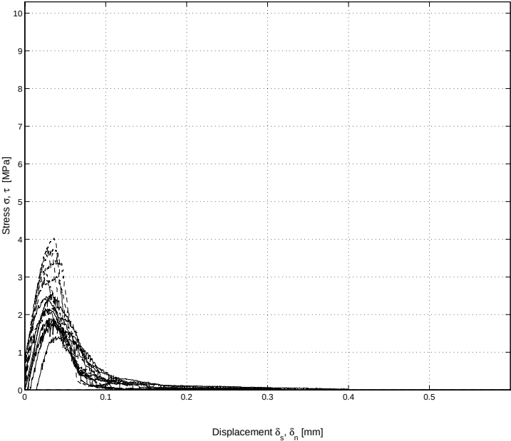
Figure 4.12: Stress-displacement, combined results for k = 2.0
