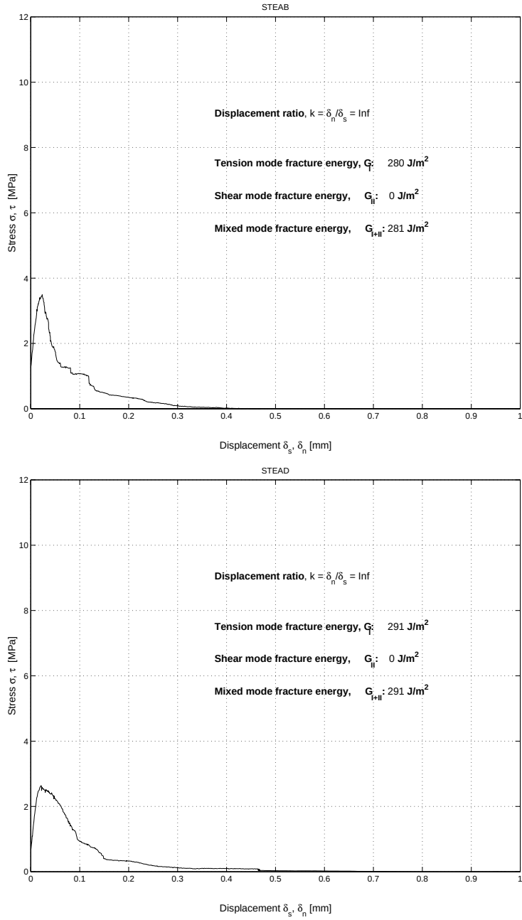
Figure B.16: Stress-displacement diagrams. Displacement ratio k = \frac{\delta_n}{\delta_s} = \infty
