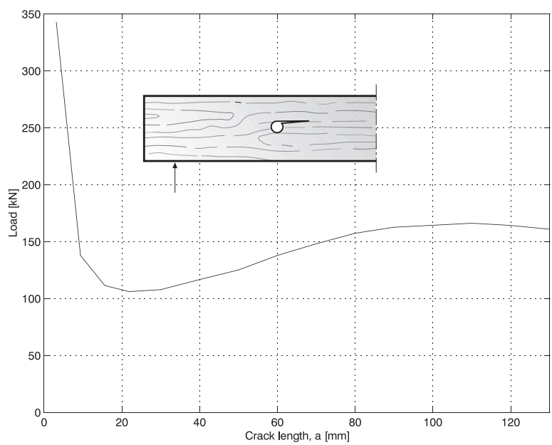
Figure 7.13: Load-bearing capacity of a beam with small internal circular hole, h = 600mm .
