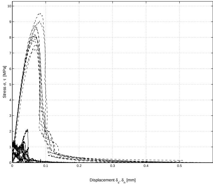
Figure 4.10: Stress-displacement, combined results for k = 0.5
