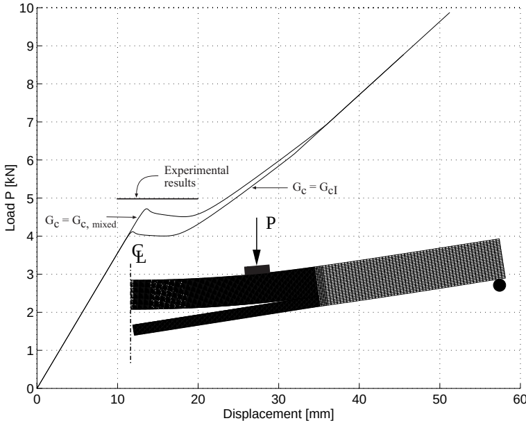
Figure 7.8: Results of four-point bending test FPB.
