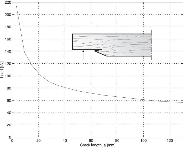
Figure 7.12: Load-bearing capacity of an tapered end-notched beam, h = 600mm .
