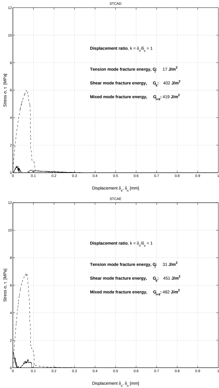
Figure B.10: Stress-displacement diagrams. Displacement ratio k = \frac{\delta_n}{\delta_s} = 1.0
