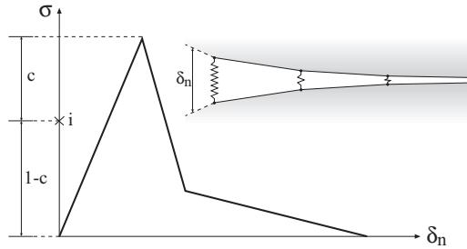
Figure 6.4: Load interval
