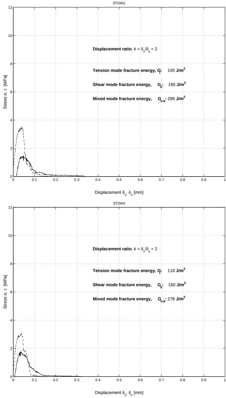
Figure B.13: Stress-displacement diagrams. Displacement ratio k = \frac{\delta_n}{\delta_s} = 2.0
