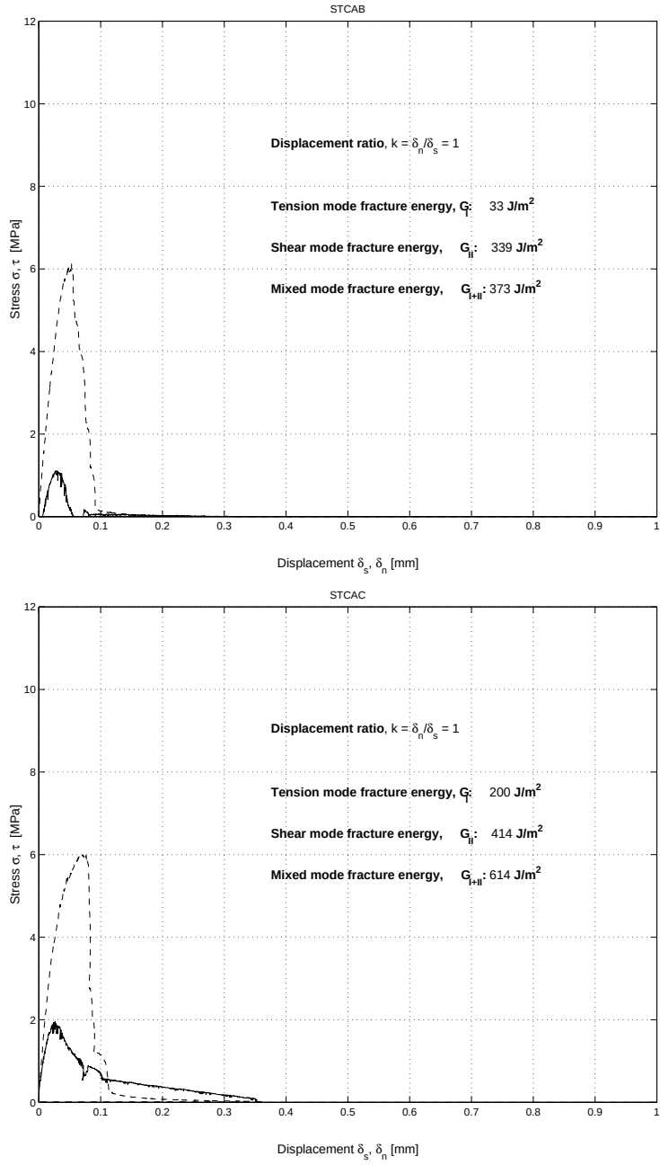
Figure B.9: Stress-displacement diagrams. Displacement ratio k = \frac{\delta_n}{\delta_s} = 1.0
