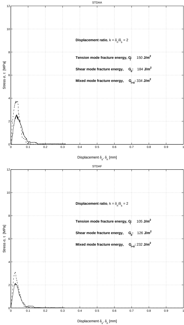
Figure B.12: Stress-displacement diagrams. Displacement ratio k = \frac{\delta_n}{\delta_s} = 2.0
