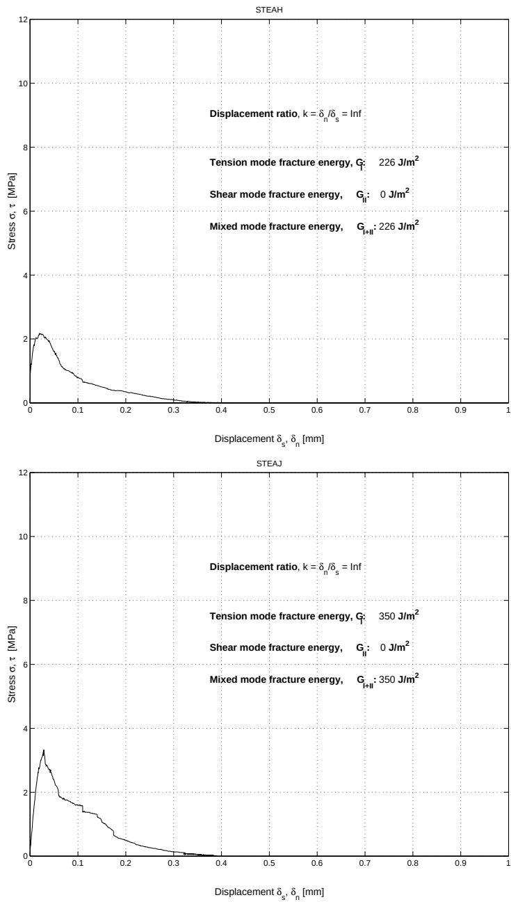
Figure B.17: Stress-displacement diagrams. Displacement ratio k = \frac{\delta_n}{\delta_s} = \infty
