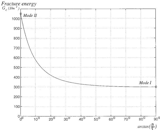
Figure C.5: Fracture criterion applied for mixed mode
