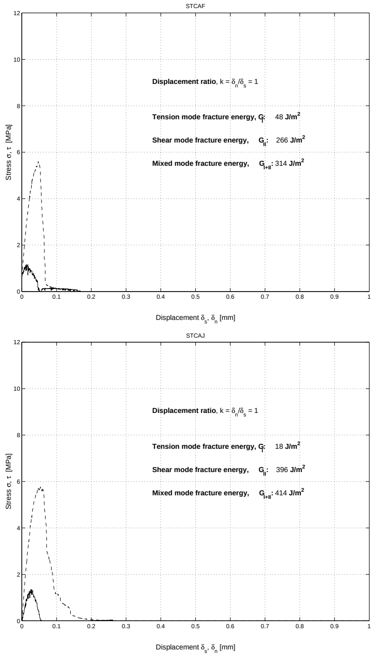
Figure B.11: Stress-displacement diagrams. Displacement ratio k = \frac{\delta_n}{\delta_s} = 1.0
