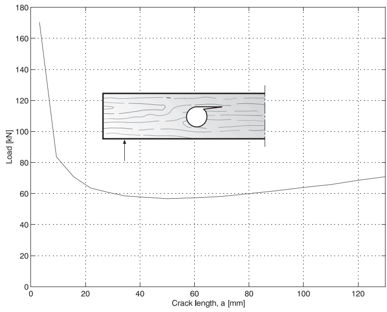
Figure 7.14: Load-bearing capacity of a beam with large internal circular hole, h = 600mm .
