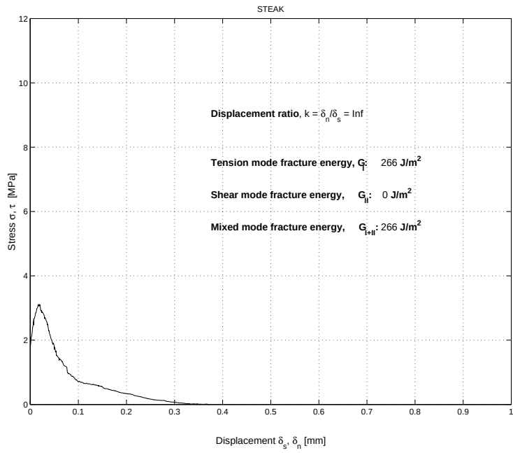
Figure B.18: Stress-displacement diagrams. Displacement ratio k = \frac{\delta_n}{\delta_s} = \infty
