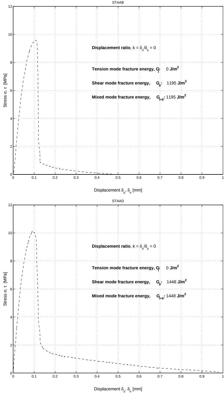
Figure B.1: Stress-displacement diagrams. Displacement ratio k = \frac{\delta_n}{\delta_s} = 0
