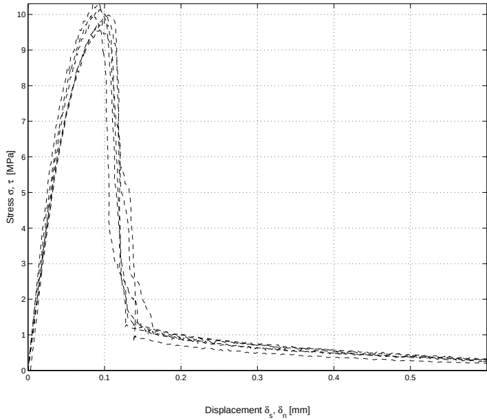
Figure 4.9: Stress-displacement, combined results for k = 0.0
