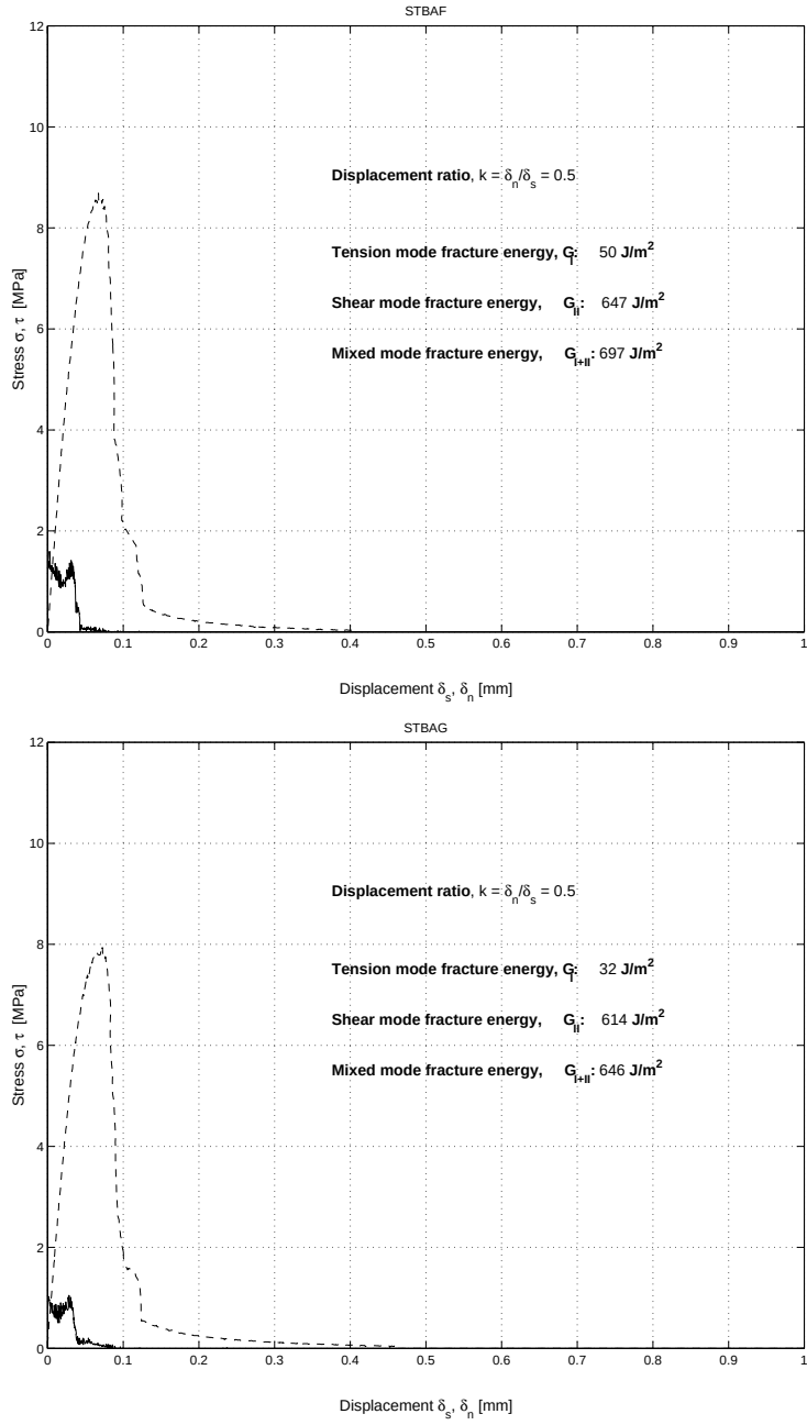
Figure B.6: Stress-displacement diagrams. Displacement ratio k = \frac{\delta_n}{\delta_s} = 0.5
