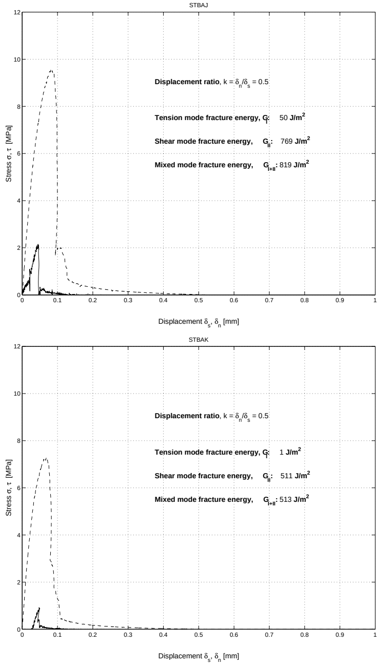
Figure B.7: Stress-displacement diagrams. Displacement ratio k = \frac{\delta_n}{\delta_s} = 0.5
