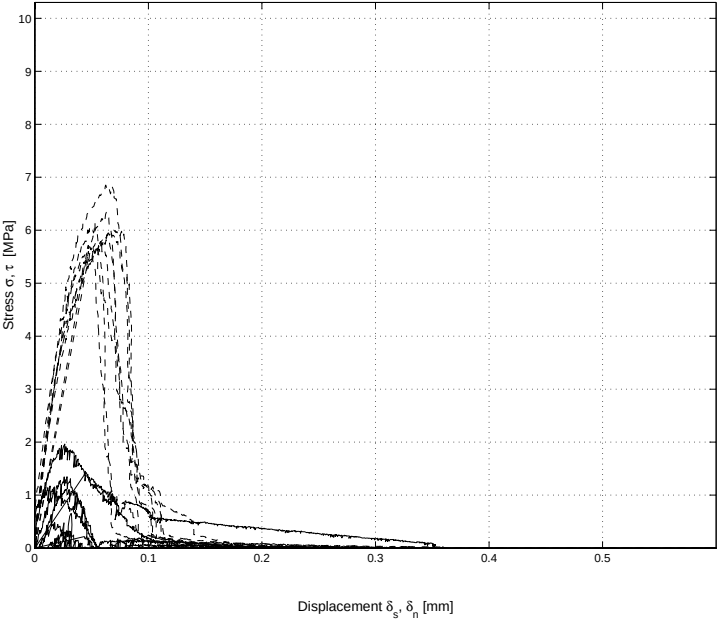
Figure 4.11: Stress-displacement, combined results for k = 1.0
