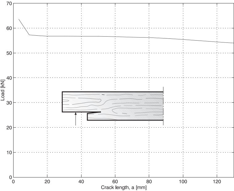
Figure 7.11: Load-bearing capacity of an end-notched beam, h = 600mm
