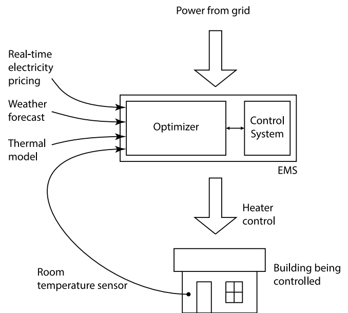
Fig. 1. Principle of the proposed energy management system.
