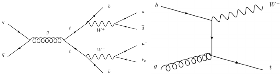
Figure 6.5.: Feynman diagrams for the production of a top quark pair (left) and W + t .
