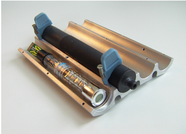
Figure 4.15.: Metal support for the PMT tubes that is used in the LUCID detector.
