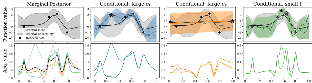
Fig. 3.3: Approximate marginal posterior after having conditioned on (\mathbf{x}^*, f^*) (top left), \alpha_{SC} using the Hellinger distance (bottom left), the three conditional truncated posteriors and their marginal contribution to the total acquisition function for the same iteration as Fig. 3.2. Conditioning on (\mathbf{x}^*, f^*) (marked as \star , drawn from function samples in dashed) introduces additional disagreement between the marginal posterior and the sampled GPs in promising regions as a result of conditioning. In the figure, we marginalize over M = 3 sets of hyperparameters and N = 2 optimizers per GP, where each optimizer’s contribution to the acquisition function is visible under its corresponding GP. Note that, since function draws are noiseless , the conditioned optimum does not need to surpass the best noisy observation in value. This phenomenon is most notable in (orange).
