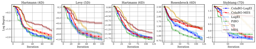
Fig. 4.5: Performance on synthetic functions with well-located priors. Both ColaBO-LogEI and ColaBO-MES offer drastic speed-ups over their vanilla variants, and offer similar performance to \pi BO. The ranking of ColaBO acquisition functions are generally consistent with their respective vanilla variants. This is most prominent on Rosenbrock (6D), where ColaBO-MES struggles similarly to vanilla MES.
