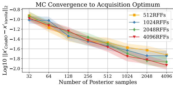
Fig. 4.4: Mean and 1/4 standard deviation of MC-induced errors of CoLaBO-LogEI relative vanilla LogEI as measured by the distance to the arg max of the acquisition function on Hartmann (3D) on 10 randomly sampled points for 40 seeds.
