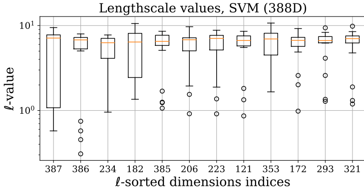
Fig. 6.8: Distribution of lengthscales values for the DSP on the 388D SVM task. Lengthscales are sorted according to their mean log value. The three last indexed dimensions (385, 386, 387) are considered particularly active [15], but are not identified as such consistently in our method. the black horizontal lines indicate upper and lower quartiles, and the orange horizontal lines indicate the median.
