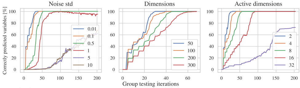
Fig. 5.3: Sensitivity analysis for GTBO. The average percentage of correctly classified variables is displayed for increasing GT iterations. The percentage is ablated for (left) various levels of output noise , (middle) number of total dimensions , and (right) number of effective dimensions . Each legend shows the configurations of the respective parameter.
