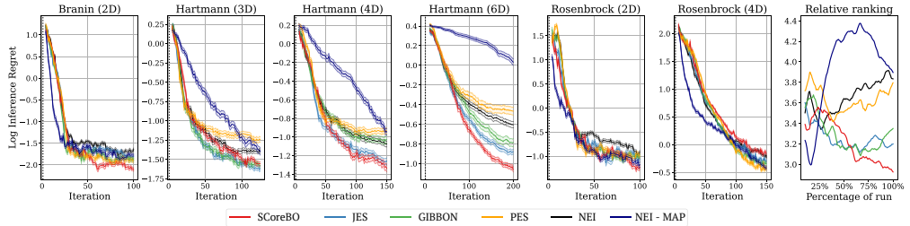
Fig. 3.6: Average log inference regret and (smoothed) relative ranking across 50 repetitions between the acquisition functions for SCoreBO, JES, MES and EI on six synthetic test functions. SCoreBO produces the best final regret on 4 out of 6 tasks, and has a substantially lower average ranking by the end of each run.
