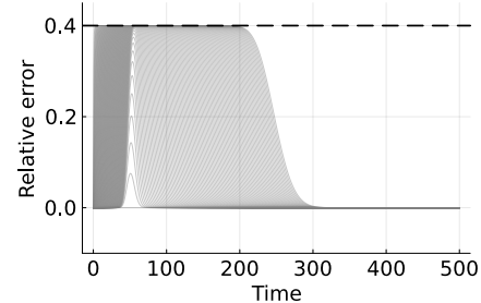
(d) Serial consensus with bidirectional feedback and N = 100 and transient \sup_t \|e_p\|_\infty = 0.400 .
