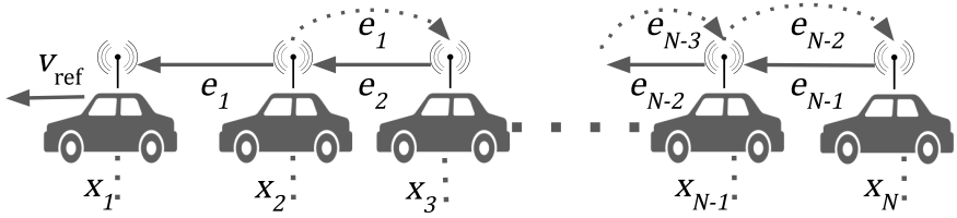
Figure 1. Illustration of vehicle formation control through serial consensus. In this example of a directed string formation, each vehicle measures the relative distance to its neighbor, and message passes its measurements to its follower.
