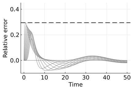
(a) Conventional consensus with symmetric position, asymmetric velocity feedback and N = 10 and transient \sup_t \|e_p\|_\infty = 0.294 .
