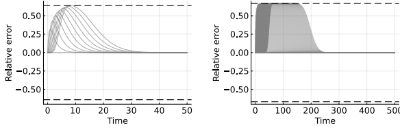
(g) Directed path, serial consensus with N = 10 and transient \sup_t \|e_p\|_\infty = 0.639 .
