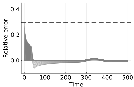
(b) Conventional consensus with symmetric position, asymmetric velocity feedback and N = 100 and transient \sup_t \|e_p\|_\infty = 0.294 .
