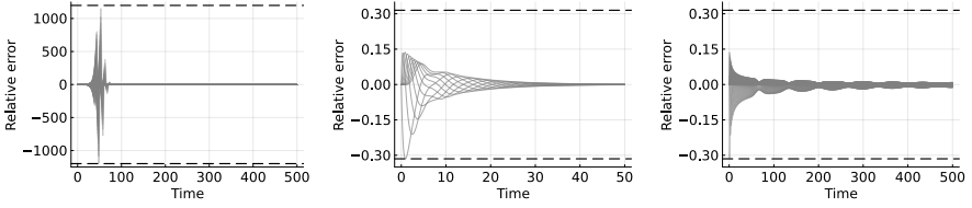
(d) Directed path, conventional consensus with N = 100 and transient \sup_t \|e_p\|_\infty = 1200 .
