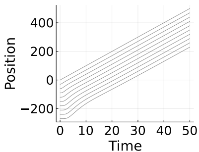
(a) Positions with N = 10 vehicles.
