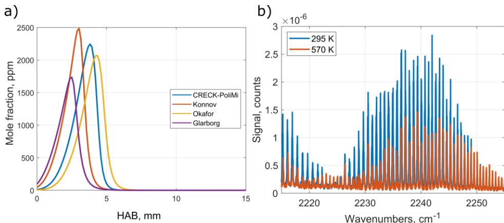
Figure 23. a) N_2O mole fractions against HAB in a \Phi = 0.9 NH_3 /Air flame as predicted by four kinetic models [28-31]. b) A comparison of the measured signal intensity of a 1000 ppm N_2O flow at two different temperatures.
