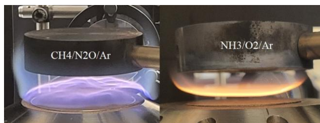
Figure 28. Photos of the two flames studied in the present experiment: the calibration CH_4/N_2O/Ar flame and the main NH_3/O_2/Ar flame.
