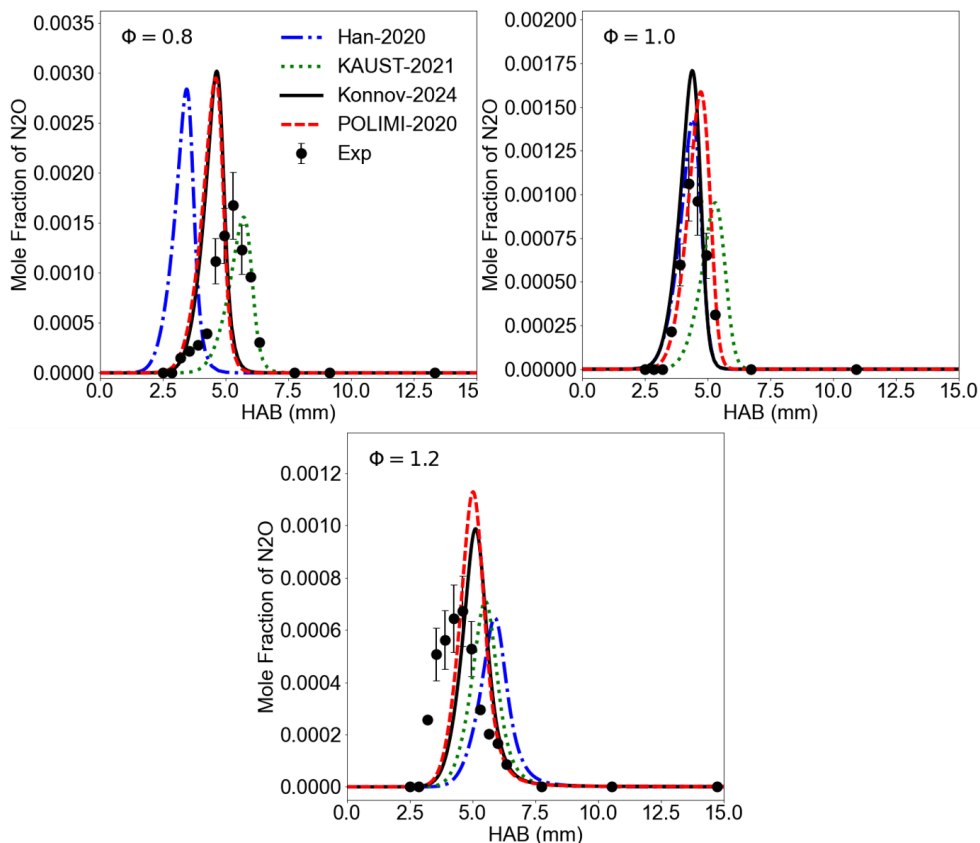
Figure 34. \text{N}_2\text{O} change with HAB. Experimental values (circles) compared with predictions of the four kinetic models (lines).
