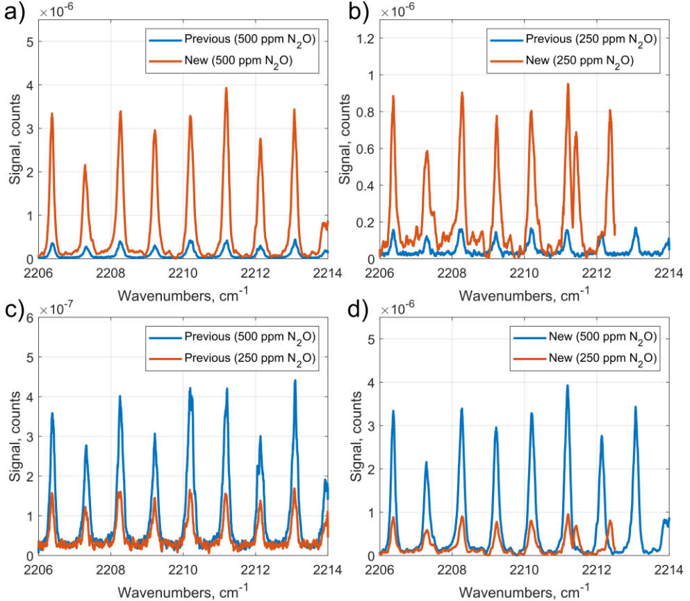
Figure 24. Signal strength comparison before and after the realignment for two \text{N}_2\text{O} flow conditions (a, b) and relative intensity comparison between these two conditions (c, d).
