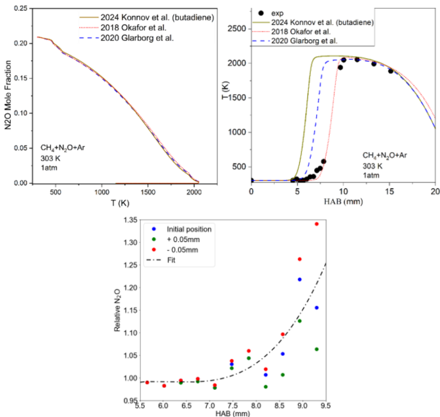
Figure 29. a) Comparison between \text{N}_2\text{O} mole fraction vs. temperature predictions of the three kinetic models [29, 36, 37]. b) Temperature profiles for \text{CH}_4 + \text{N}_2\text{O} + \text{Ar} calibration flame. Experimental values (circles) compared with simulations (lines) [29, 36, 37]. c) Ratio between \text{N}_2\text{O} mole fraction modelling predictions [29] and experimental data evaluated using a room-temperature \text{N}_2\text{O} cross-section value. The graph represents the temperature dependence of the \text{N}_2\text{O} cross-section.
