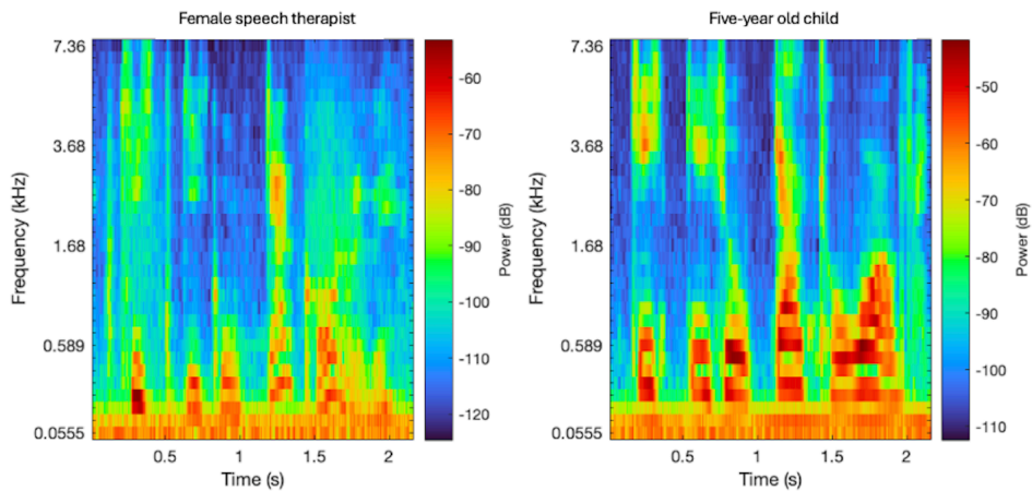
Figure 1 – Mel spectrograms.
