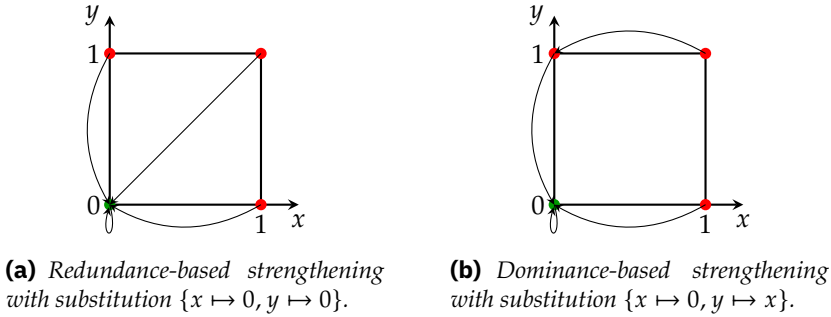
Figure 2: Example for how the substitution patches the assignment for database C \cup \mathcal{D} = \emptyset and order \mathcal{O}_\geq(i_1, i_2, k_1, k_2) = \{2i_1 + i_1 \geq 2k_1 + k_2\} loaded over the literals \vec{z} = x, y to a solution satisfying also the constraint \bar{x} + \bar{y} \geq 2 .
