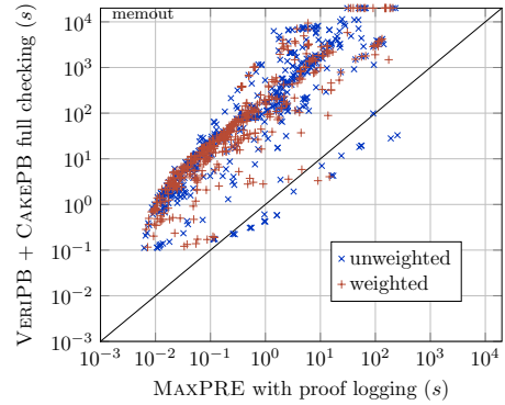
Figure 7: MAXPRE vs. combined proof checking running time.
