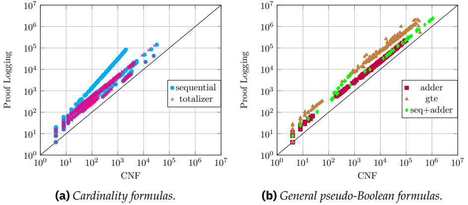
Figure 10: Comparison between CNF file size and proof logging file size in KiB.
