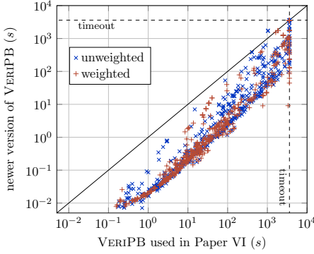
Figure 3: VERiPB version used in Paper VI vs. latest VERiPB version.
