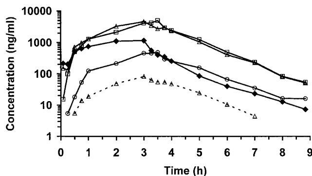
Fig. 5. The plasma concentrations of pentoxifylline and its metabolites during and after the intravenous infusion of 600 mg of the drug over 3 h in one subject. Key: filled diamonds: pentoxifylline, open triangles with dashed line: (R)-M1, with continuous line: (S)-M1, open circles: M4, and open squares: M5.
