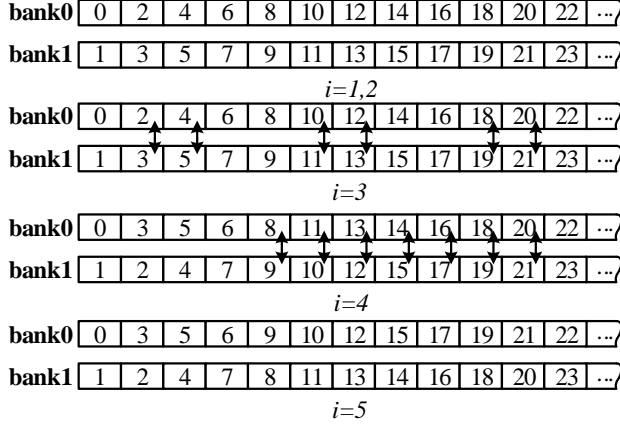
Figure 6.11. Data mapping scheme for N=2 bank sorting. Numbers within boxes denote indexes. Bi-direction arrows denote data re-allocation at the end of each phase.
