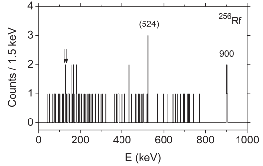
FIG. 3. Energy spectra of \gamma rays in coincidence with the recoil electrons, which had a spontaneous fission event following the electron ( r - e - f ). The arrows show the locations of the most intense Rf x-ray peaks.
