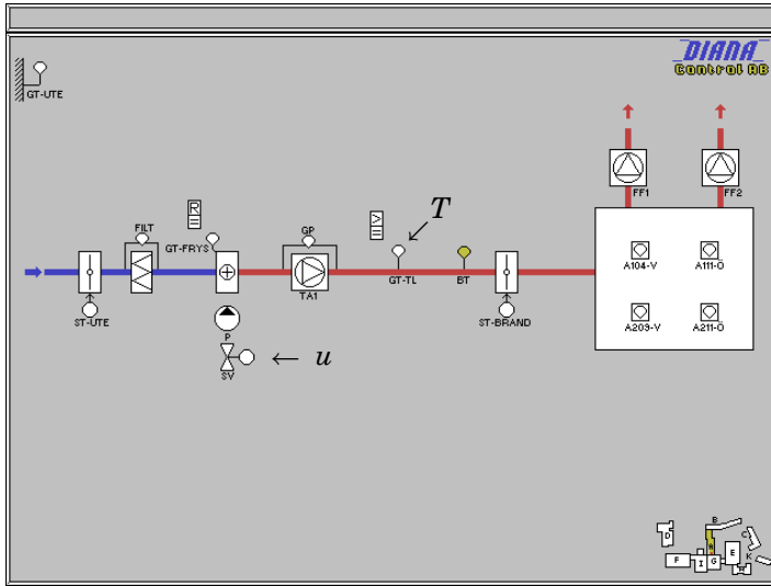
Figure 16. The air temperature control loop. The water flow to the heat-exchanger is controlled by a valve via the control signal u . The output is the air temperature T after the fan.
