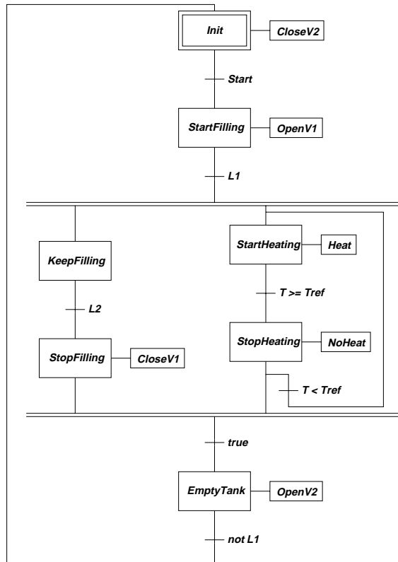
Figure 6. Grafset for the controller of a boiler process. This figure is generated by the PAL compiler.
