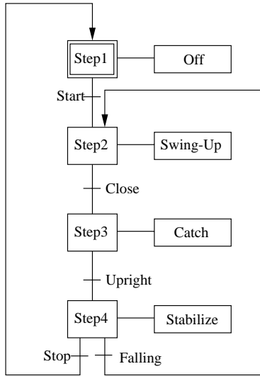
Figure 6. The Grafset which describes the switching rules for the hybrid pendulum controller.
