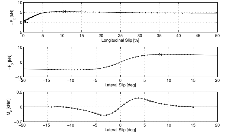
Figure 5.4 Pure-slip measurement data (dots) with Magic Formula parametrization (solid lines) for the forces and interpolation of raw data for the aligning moment. The limit slips calculated from (5.25) are marked by crosses in the two upper plots.
