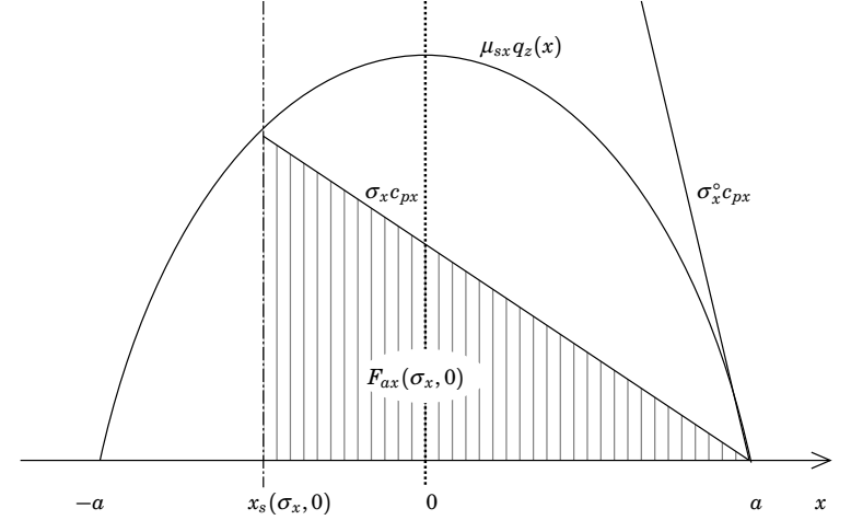
Figure 4.4 Illustration of the adhesive tire-force for pure longitudinal slip. The elastic deformation force for an element at x in the adhesive region depends linearly on x as c_{px}\sigma_x(x - a) , where the slope is proportional to the slip \sigma_x . The transition from adhesion to slide occurs at the intersection of the lines at the break-away point x_s . For slips \sigma_x > \sigma_x^\circ full sliding occur in the contact area since there is then no intersection.
