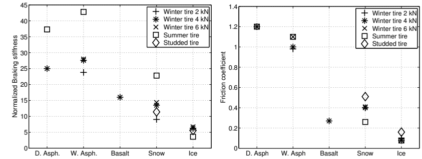
Figure 7.9 Visualization of the results from Table 7.1. The normalized tire stiffnesses and friction coefficients of the tested tires at different loads are plotted as functions of the surface.
