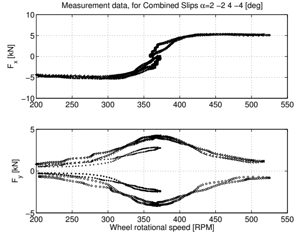
Figure 5.2 Available measurement data for combined slip. Longitudinal and lateral force at F_z=5.3 or 5.5 kN, see comment in text.
