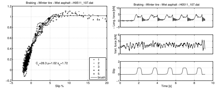
Figure 7.2 Measurement data from Hållerød showing results from the winter tire on wet asphalt with a vertical load of 4 kN. To the left: Adaptation of the brush model. The normalized brake force is shown as a function of the slip, \lambda . To the right: Recorded signals showing the test sequences in the measurement file.
