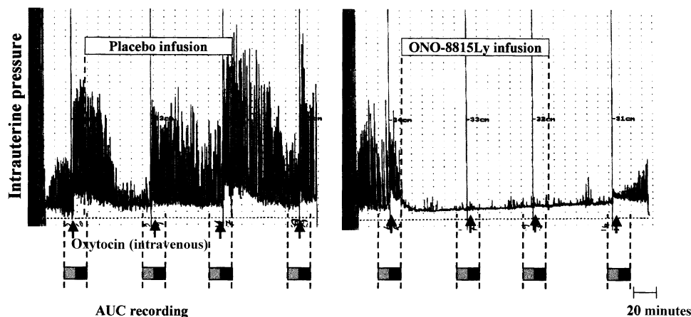
Fig. 2. Representative recordings of the effect of placebo (left) and ONO-8815Ly at an infusion rate of 8 µg/minute (right) on intrauterine pressure in a healthy woman at menstruation. Intravenous bolus injections of oxytocin in a dose of 50 pmol/kg body weight were given on four occasions each time (indicated). The AUC was calculated for 10 minute periods before and after each oxytocin injection (also indicated).
