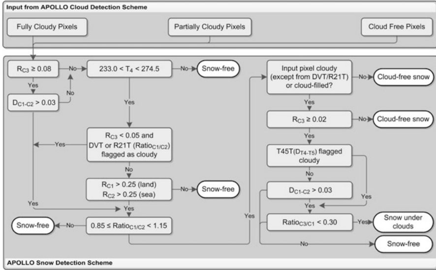
Fig. 4.2 APOLLO scheme to detect snow cover from AVHRR data ( RC_3 : Reflectance in channel 3; DC_1-C_2 : Difference between channel 1 and channel 2; T_4 : brightness temperature in channel 4; RatioC_1/C_2 : ratio between channel 1 and channel 2; DVT : dynamic visible threshold; R_21T : ratio between channel 1 and channel 2 – cloud test; T_45T : difference between brightness temperatures of channels 4 and 5)
