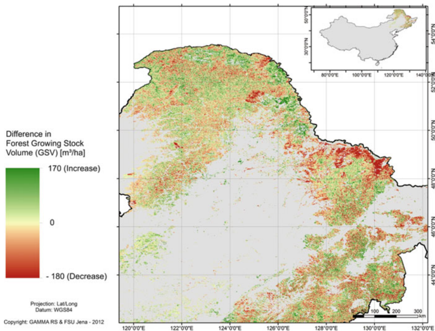
Fig. 16.21 Growing Stock Volume (GSV) change map from estimates obtained with the BIOMASAR algorithm using Envisat ASAR ScanSAR images acquired in 2005 and 2010 (Schmullius et al. 2012). The study area has a total coverage of about 540,000 km 2 including forest and shrubland areas according to the GLC2000 land cover information. The map is characterized by several changes through fire, logging and re-forestation. The GSV estimated with the BIOMASAR algorithm presents an uncertainty quantified on the order of 10 % regardless of the GSV level as proven with comparable inventory data from Siberia
