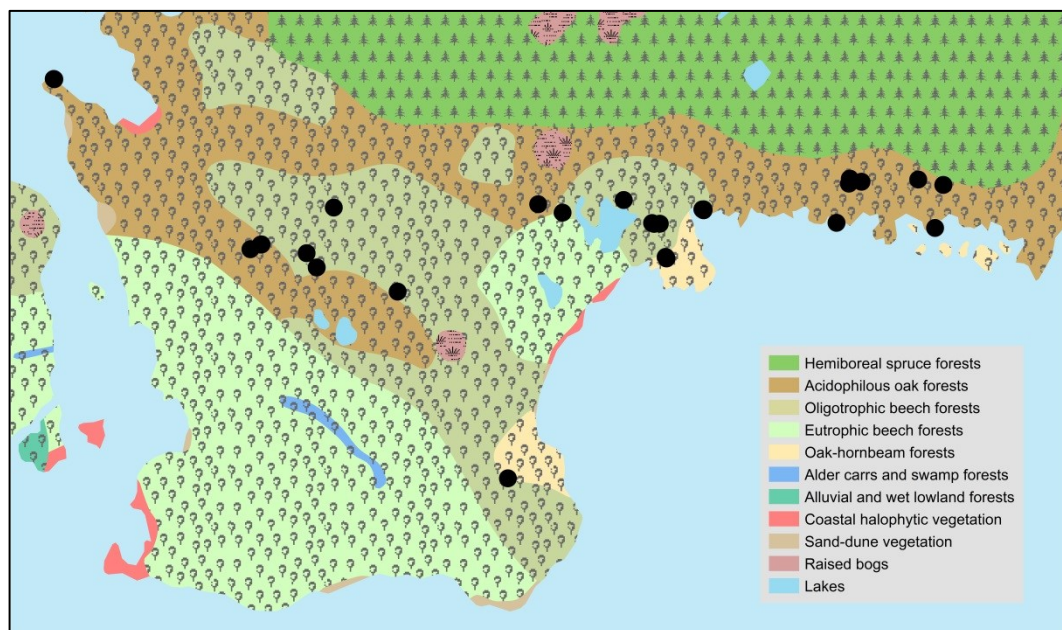
Figure 7. Potential natural vegetation according Bohn & Neuhausl (2000/2003) and distribution of Lobaria pulmonaria in the study area.
