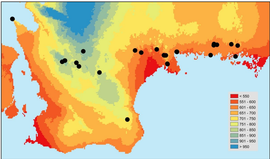
Figure 6. Annual precipitation (in mm) according Fick & Hijmans (2017) and distribution of Lobaria pulmonaria in the study area.
