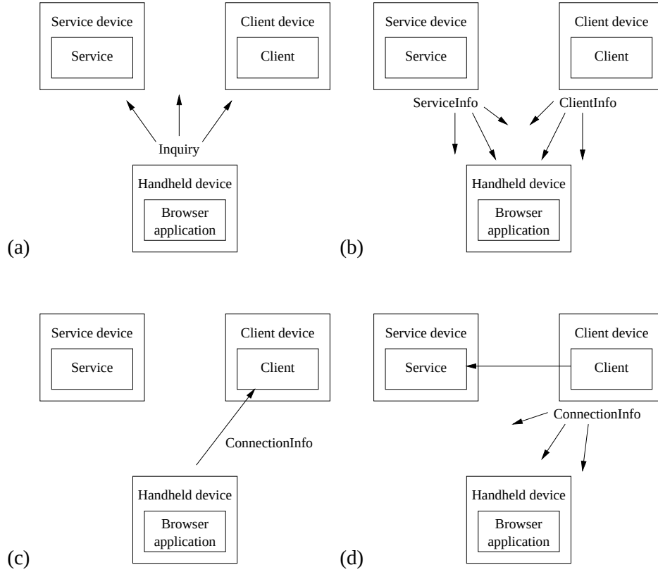
Figure 4: Discovering and connecting services.
