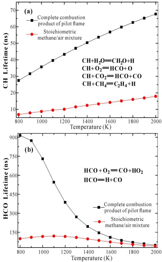
Figure 2. Numerical simulations of (a) CH and (b) HCO lifetimes at various temperatures in a closed homogeneous reactor with a mixture composition corresponding to that of combustion product of the pilot flame (squares), and alternatively a stoichiometric methane/air mixture (circles). A number of major reactions responsible for CH/HCO consumption under the simulated conditions are shown.
