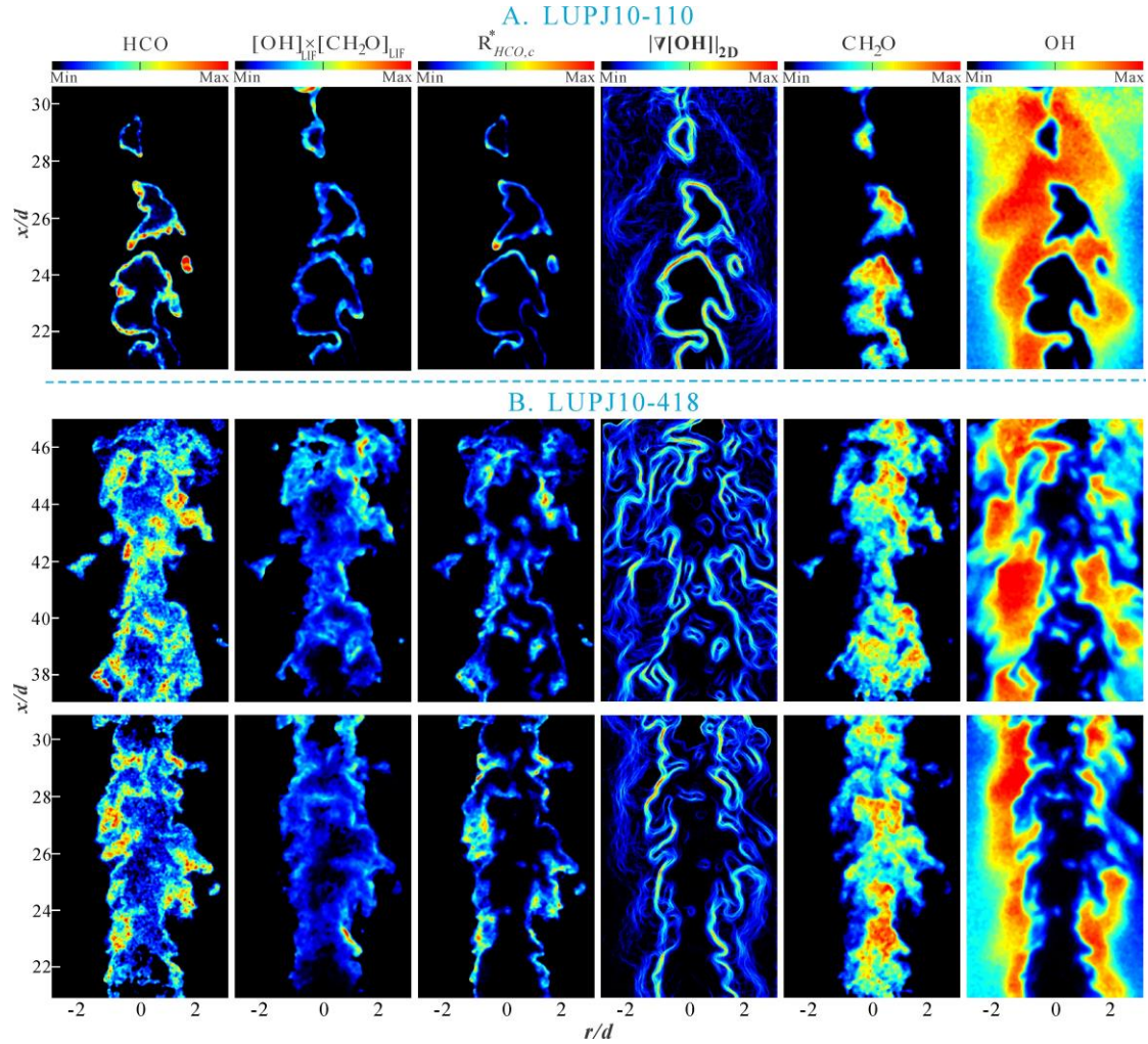
Figure 4. Examples from the HCO/CH 2 O/OH dataset: simultaneous snapshots of reactive scalars (i.e. HCO, CH 2 O and OH), product of OH and CH 2 O ([OH] LIF ×[CH 2 O] LIF ), OH gradient ( |\nabla[\text{OH}]|_{2D} ) as well as the relative reaction rate R_{HCO,c}^* for flames LUPJ10-110 and LUPJ10-418.
