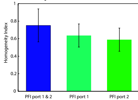
Figure 76. Homogeneity index for different PFI strategies. The bars indicate the 95% confidence interval for the mean values.
