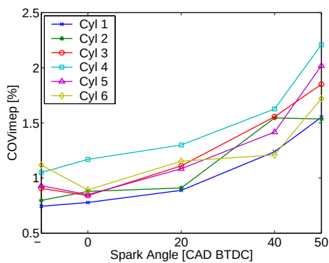
Figure 22. COV_{imep} for HCCI with and without spark assistance for ~3,4 bar IMEP at 1500 rpm.
