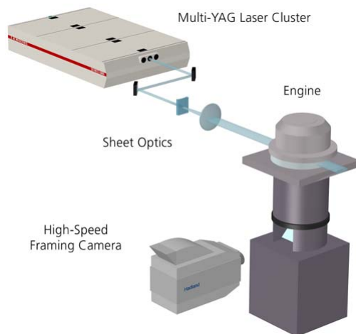
Figure 2. A schematic of the optical setup.
