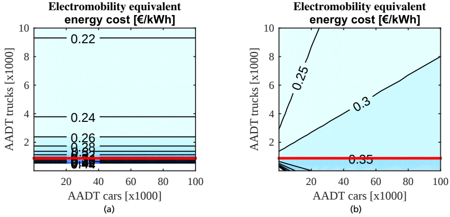
Figure 5.12: Electromobility equivalent energy cost C_{emo} for overhead lines ERS only for trucks; cars remain on fossil fuels.
