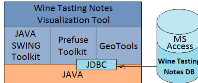
Fig. 5.11 Software architecture of the tool.
