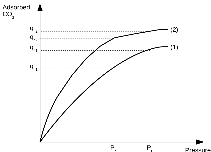
Figure 9 Two generic adsorbant isotherms showing the partial pressure of CO 2 in the gas streams at feed pressure (high) and regeneration pressure (low). \Delta q equals the separating capacity for one column cycle. Image adapted from (Grande 2011).
