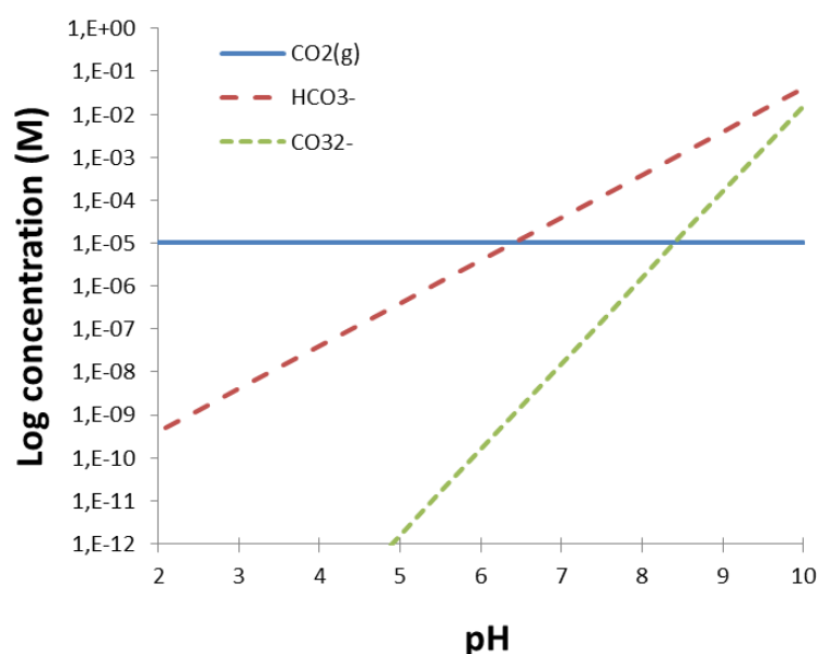
Figure 1 The calculated pH diagram for the carbonate system in the liquid-phase in the desorption column. Water was assumed to be equilibrated with the atmosphere ( p_{CO_2} = 10^{-3.5} atm) and the constants pK_H = 1.5 , pK_{a1} = 6.4 and pK_{a2} = 10.4 were used (all valid at 25°C). In the absorption column p_{CO_2} is around 10^{0.5} atm which will increase all concentration approximately 10^4 times.
