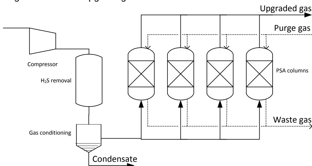
Figure 6 Process diagram for upgrading of biogas with PSA. H 2 S and water vapour is separated from the raw biogas before it is fed to the adsorption column. Multiple columns work in parallel cycles for a continuous process. Figure adapted from (De Hullu et al. 2008)
