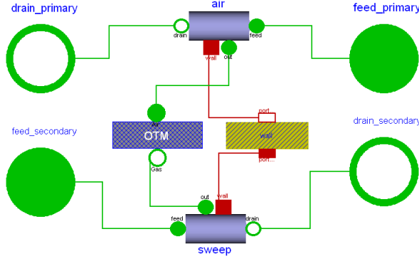
Figure 5: Model diagram view of the membrane reactor model: OTM -Oxygen transfer membrane, Air -air flow model, Sweep -exhaust gas flow model, wall -wall model for heat transfer.
