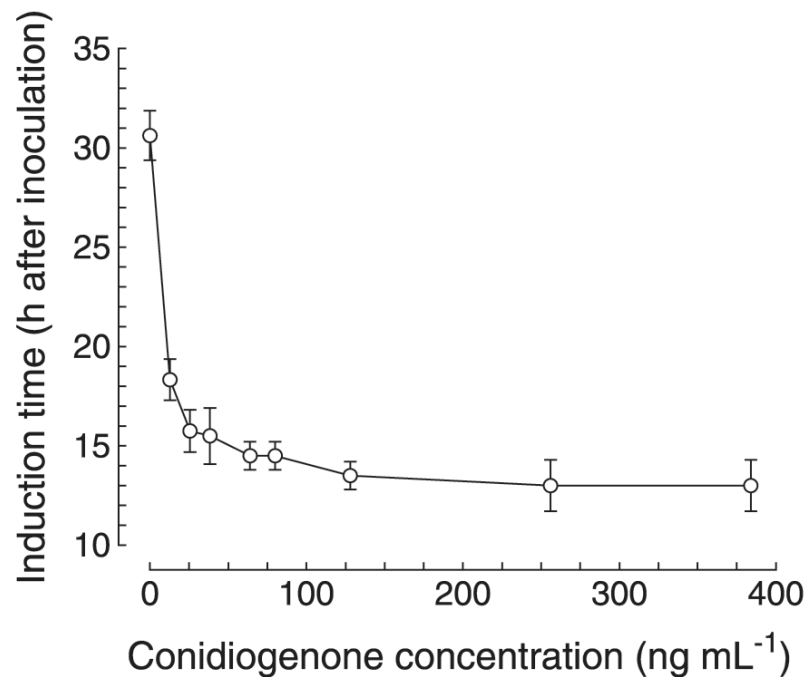
Figure 2.5. Effect of conidiogenone concentration on the conidiation induction time in the absence of calcium in the culture medium. Increasing concentrations of conidiogenone were added to fresh F medium (with no calcium added), and the time at which conidiation induction occurred was determined. The threshold concentration required to induce conidiation was determined as the lowest concentration which allowed induction to occur at the earliest time.
