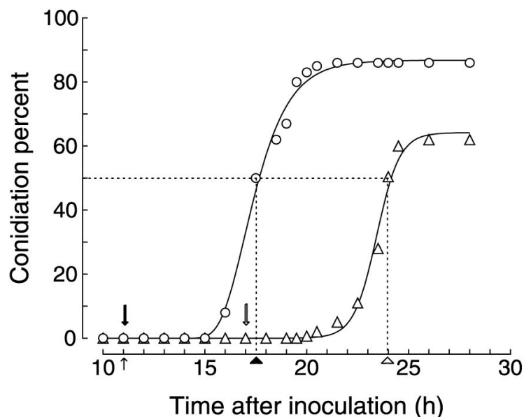
Figure 2.2. Temporal appearance of conidium-bearing tips in cultures of P. cyclopium . The percentage of conidiating tips is expressed as the conidiation percent. Assays were carried out in shaken flask cultures inoculated with 10^{13} conidia/ml. The points of 50% conidiation, taken as the reference point at which conidiation was considered to have been reached, are indicated by dotted lines. Triangles represent growth in fresh F medium and circles represent growth in mF medium. The mF medium was prepared by growing the fungus in a 10 liter fermenter for 36 h with an inoculum of 10^6 conidia/ml.
