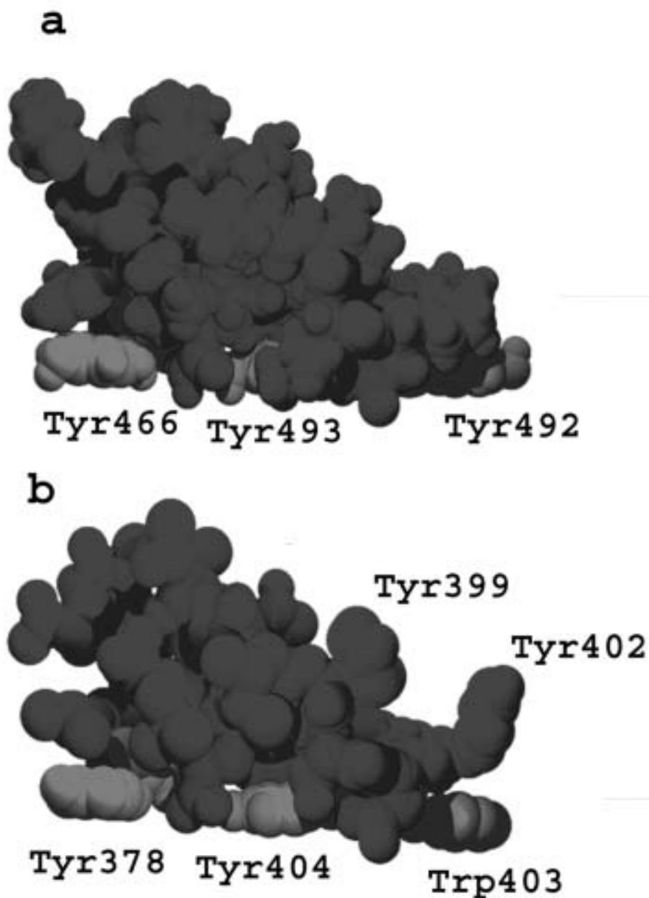
Figure 12. a. Structure of the CBM from TrCel7A. b. Model of the CBM from TrMan5A, based on the structure of the CBM from TrCel7A. The numbers of the aromatic residues on the flat sides of the CBM from TrCel7A and the model of the TrMan5A CBM are indicated. The numbers of the tyrosines on the rough side of the model of the CBM from TrMan5A are also indicated.
