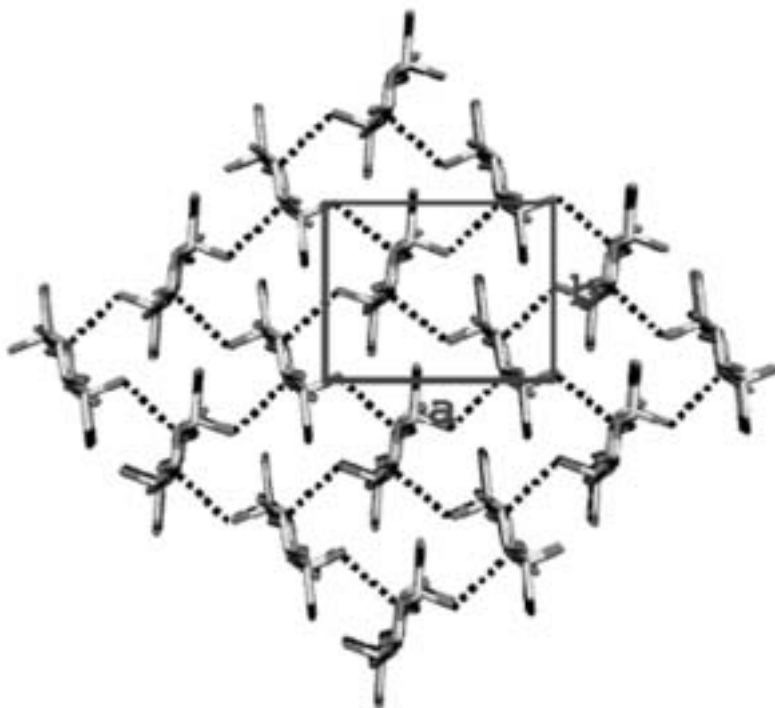
Figure 14. Structure of mannan I viewed as a projection of the unit cell onto the ab plane. The unit cell dimensions are a=8.92 Å, b=7.21 Å and c=10.27 Å. Adapted from [222].
