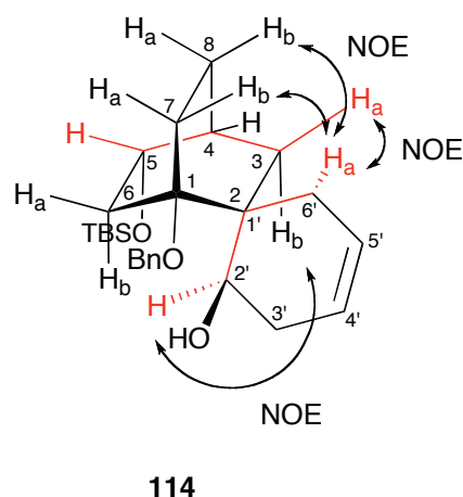
Figure 14. Spiro bicyclic compound 114 with important correlations.
