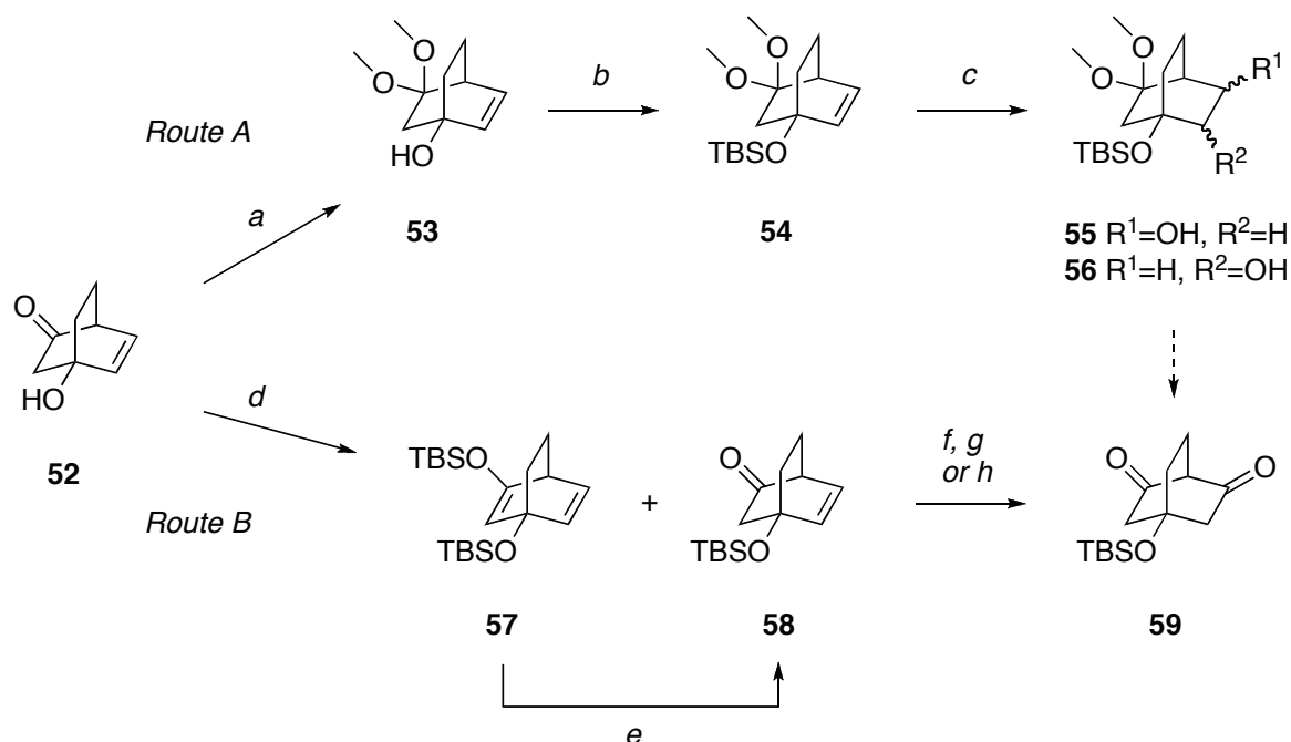
Scheme 8. Synthesis of diketone 59 . Reaction and conditions: (a) trimethylorthoformate, p -TsOH (cat.), MeOH, rt, 24 h, quant. (b) TBSCl, NaH, THF, 0 °C→rt, 12 h, 52% from 52 (c) i. BH_3 \cdot THF , THF, 0 °C→rt, 3 h ii. 2M NaOH, 30% H_2O_2 , rt, 12 h, 55 0%, 56 39% (d) TBSCl, 2,6-lutidine, DCM, 0 °C, 3 h (e) 1M HCl, THF, rt, 1 h, 70 % from 52 (f) i. BH_3 \cdot THF , THF, 0 °C, 3 h ii. 2M NaOH, 30% H_2O_2 , rt, 12 h (g) Jones's oxidation, 64% (h) i. BH_3 \cdot THF , THF, 0 °C, 3 h ii. TPAP, NMO, 4Å MS, DCM, rt, 4 h, 42%.
