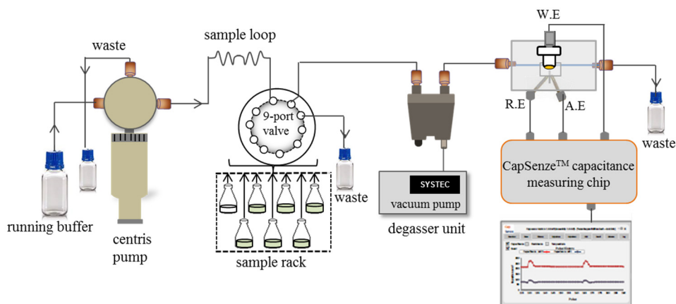
Fig 4.10: Illustration of the component of the Capsenze™ capacitive biosystem.
