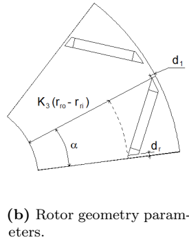
Figure 2.9: Geometric parameters evaluated in the machine optimization.
