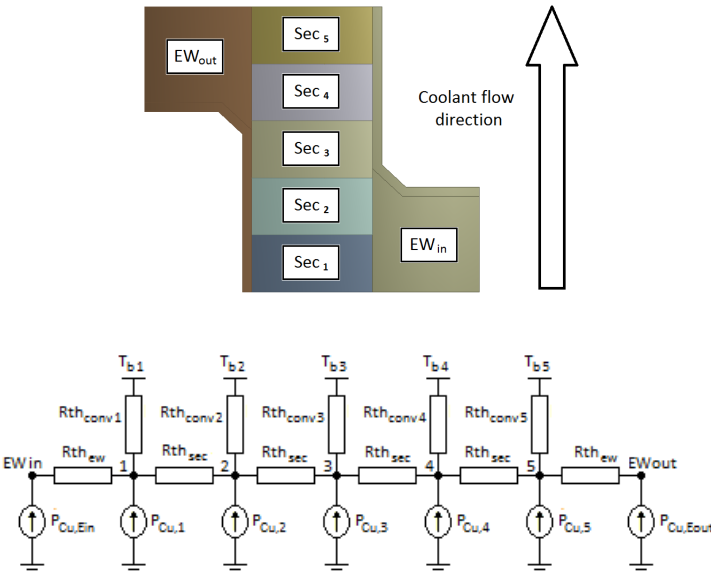
Figure 4.5: Lumped parameter model of a single turn.
