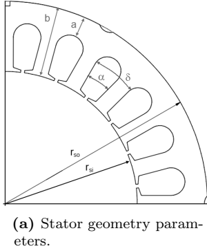
Figure 2.9: Geometric parameters evaluated in the machine optimization.
