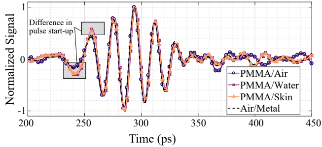
Figure 6.5: The reflection of mm-wave pulses at different material interfaces, normalized to its maximum. The reflection of the Air/Metal interface is assumed to be the undistorted incident signal. The reflection on the PMMA/Air interface is basically undistorted compared to the reference. Reflections from the PMMA/Water and PMMA/Skin interface are clearly distorted, resulting in a difference in the pulse start-up
