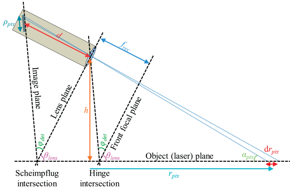
Figure 4.9 Schematic illustration of how the Scheimpflug principle and Hinge rule are implemented in Scheimpflug lidar. When the planes align in the Scheimpflug- and Hinge intersection, infinite focal depth along the laser beam is achieved. Thus, each pixel on the sensor monitors a specific section of the laser beam with sharp focus.
