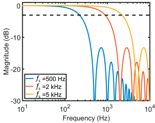
Figure 3.3 Bode plot for an integrating detector, modelled with a sinc function. According to the model, a 500 Hz sample rate yields a 220 Hz bandwidth, a 2 kHz sample rate yields a 880 Hz bandwidth and a 5 kHz sample rate yields a 2.21 kHz bandwidth. Unlike TIAs, integrating sensors have adjustable bandwidths.
