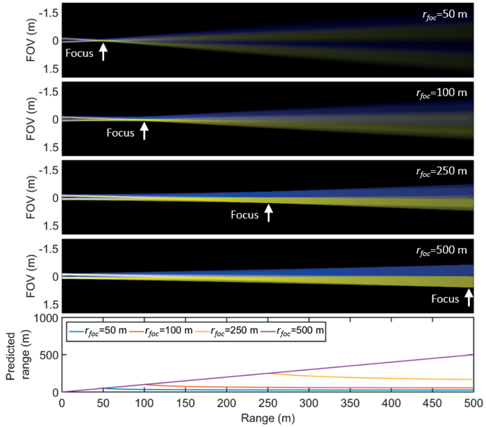
Figure 4.8 The effect of the focal distance on the range prediction. The FoV of two adjacent sensor elements is simulated with raytracing. Four cases are presented in which the sensor is focussed at different distances. The bottom panel shows the predicted range compared to the actual range in the simulation, demonstrating that the passive ranging equation is invalid beyond the focal distance of the sensor.
