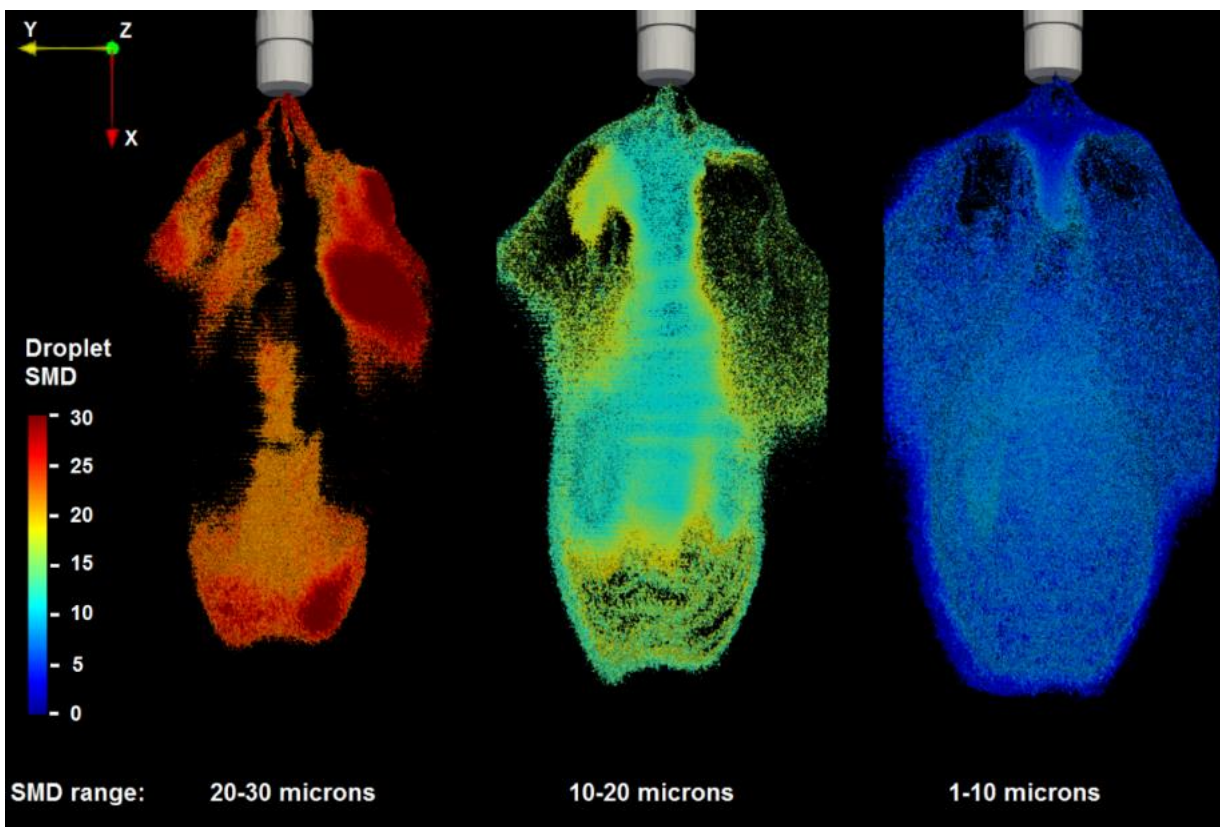
Fig. 9. Back view: 3D map of the DISI spray plotted as the function of droplet SMD range, for a better insight into the inner structure of the spray: 20-30 \mu\text{m} (left), 10-20 \mu\text{m} (middle), and 1-10 \mu\text{m} (right).
