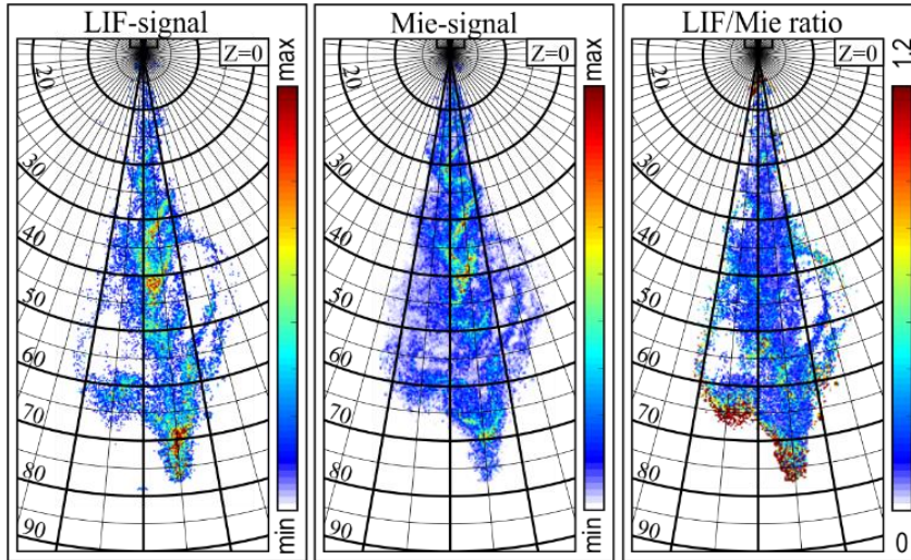
Fig. 4. Instantaneous images of LIF, Mie and the corresponding LIF/Mie ratio for ethanol DISI spray at 2552 \mu\text{s} aVSOI.
