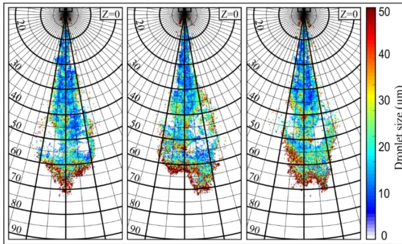
Fig. 5. Instantaneous absolute SMD maps in ethanol DISI sprays at 2552 \mu\text{s} aVSOI. The regions between Y = 20\text{--}60 mm below the nozzle exit show droplet sizes in the range 5–45 \mu\text{m} . In the regions between Y = 60\text{--}75 mm, the droplet SMD ranges from 20–50 \mu\text{m} .
