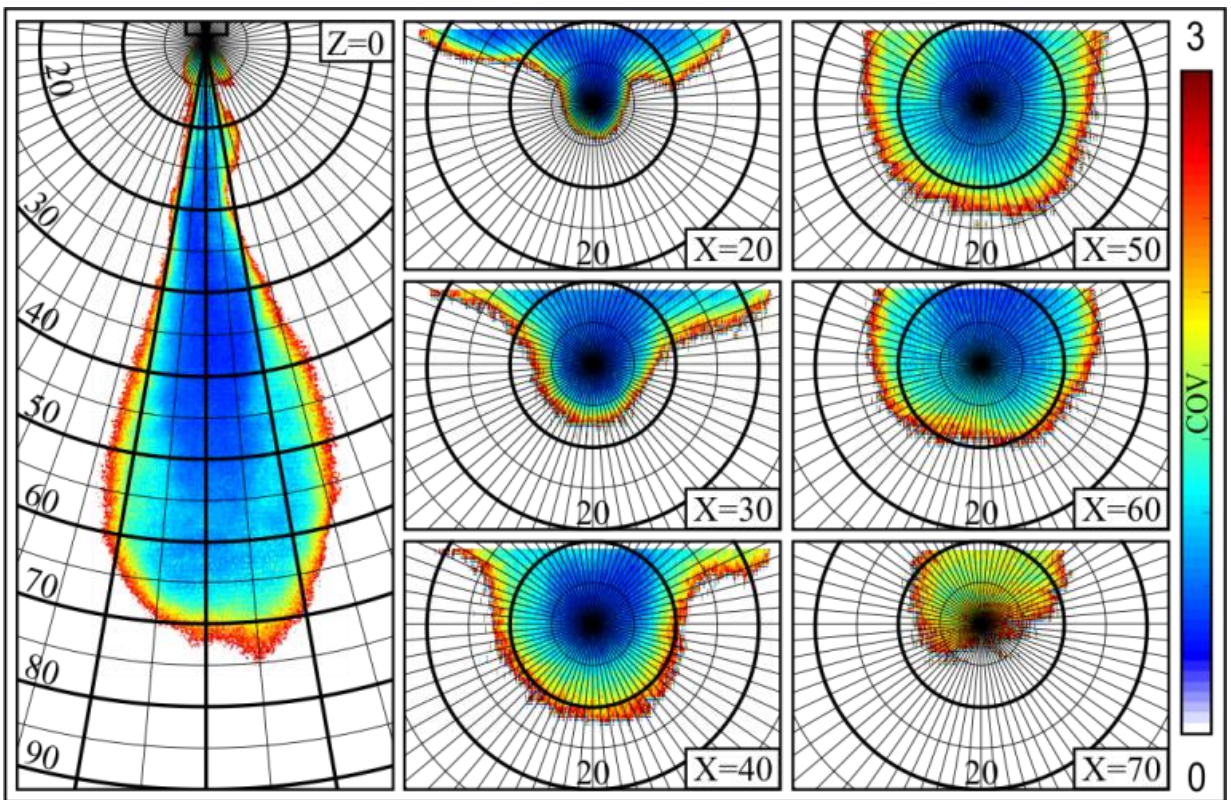
Fig. 11. COV of SMD cross-sections maps for ethanol DISI sprays. The COV maps show strong cyclic variations near the spray edges and spray front. Recording time was at 2552 \mu\text{s} aVSOI.
