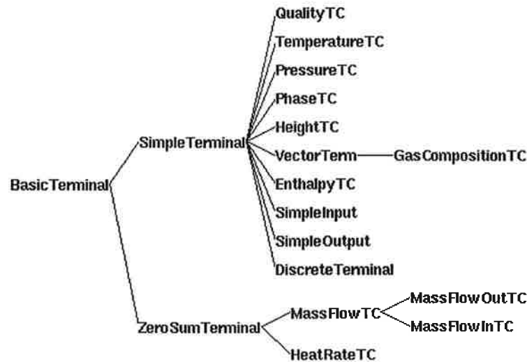
Figure 8. The class hierarchy of basic terminal classes in the K2 terminal library.
