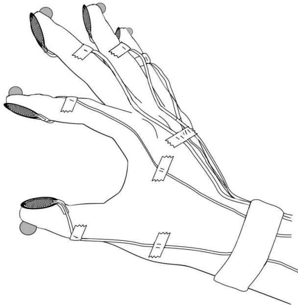
Figure 2: An illustration of a hand with attached force sensors.
