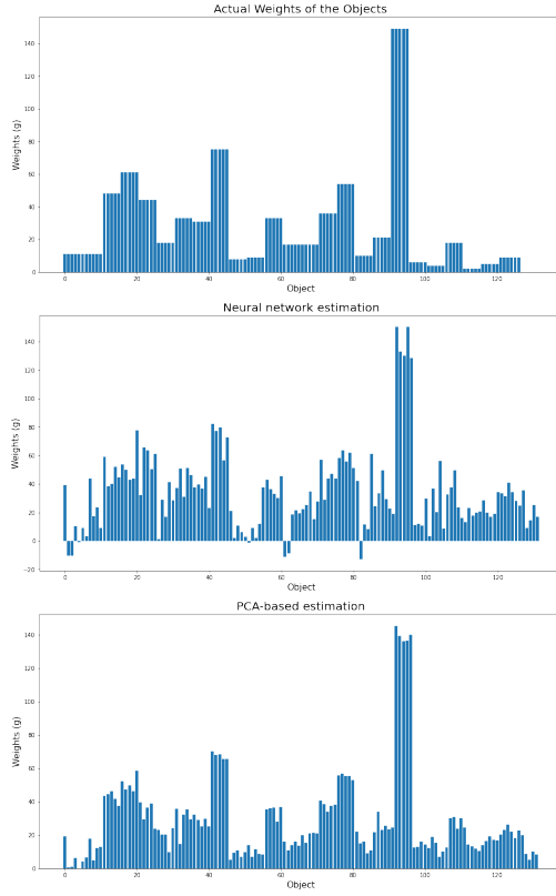
Figure 16: TOP. The actual weights of the objects. MIDDLE. The weights of the objects estimated using the neural network. BOTTOM. The weights of the objects estimated using the first principal component (scaled to the mean of the actual data for comparison). The PCA-based method is clearly less noisy.
