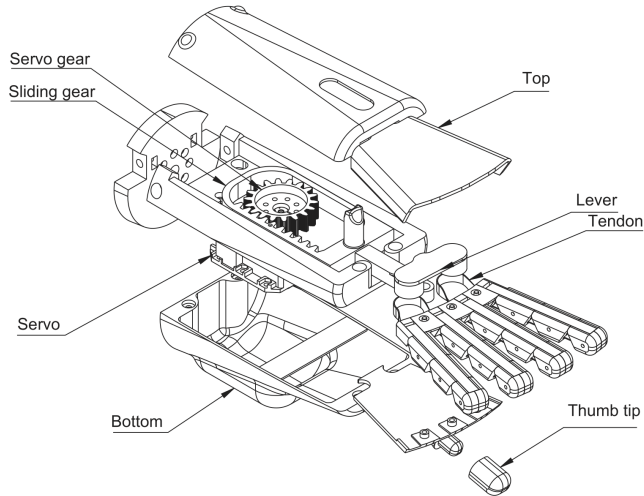
Figure 2: The design of the robot hand used in the experiments. The four movable fingers are controlled by a single servo through a gear rack that drags rubber tendon using a whippletree mechanism within the palm of the hand to distribute the force from the servo to the different fingers.
