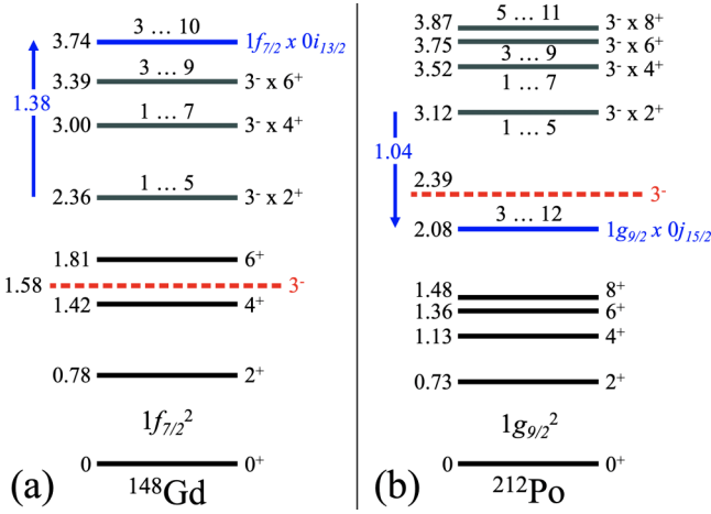
FIG. 12. (a) Members of the 1f_{7/2}^2 multiplet (black) and unperturbed energies of the 1f_{7/2} \times 3^- states (gray) in ^{148}\text{Gd} . The position of the 3^- phonon state in the ^{146}\text{Gd} core is indicated by a red dashed line while the unperturbed position of the 1f_{7/2} \times 0i_{13/2} multiplet is shown in blue. (b) Members of the 1g_{9/2}^2 multiplet (black) and unperturbed energies of the 1g_{9/2} \times 3^- states (gray) in ^{212}\text{Po} . The position of the 3^- phonon state in the ^{210}\text{Po} core is indicated by a red dashed line while the unperturbed position of the 1g_{9/2} \times 0j_{15/2} multiplet is shown in blue. The numbers above the gray and blue lines indicate the spin range of the multiplets.
