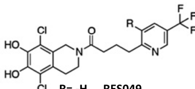
R= -H RES049 R= -Me RES155 R= -Cl RES137
