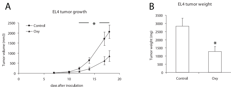
Figure 2. OX inhibits EL4 lymphoma growth in vivo . A: Anti-tumor effect of OX in EL4 tumors inoculated (s.c.) into wild type mice. OX was administered p.o. at 30 mg/kg/day 7 days/week from day 1 throughout the experiment. Each data point represents mean \pm SEM (n=10; *p<0.05, Mann Whitney U). Control animals received only water. B: Tumor weights (*p<0.05; Mann Whitney U). doi:10.1371/journal.pone.0063012.g002
