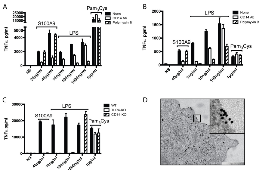
Fig 5. CD14 is essential for the S100A9-induced cytokine response. (A,B) Blocking of CD14 inhibits S100A9-induced cytokine response. (A) THP-1 cells ( 1 \times 10^6 /ml) or (B) peritoneal wash cells ( 1 \times 10^6 /ml) were pre-incubated with (A) mouse-anti-human CD14 blocking antibody ( 5 \mu\text{g/ml} ), (B) rat-anti-mouse CD14 blocking antibody ( 10 \mu\text{g/ml} ), (A,B) polymyxin B ( 50 \mu\text{g/ml} ) or medium (NS) for 30min, as indicated. The cells were subsequently cultured in medium (NS) or stimulated with indicated concentration of S100A9 protein, LPS or TLR2-stimulator Pam 3 Cys ( 1 \mu\text{g/ml} ); cells were stimulated with 40 \mu\text{g/ml} S100A9 in (B). Supernatants were harvested after (A) 4hrs or (B) 24 hrs of culture and TNF \alpha concentration determined using CBA assay. Results from one representative experiment out of 3 (A) and 2 (B) independent experiments are shown. (C) BM-DCs from indicated mouse strains were stimulated with 40 \mu\text{g/ml} moS100A9, or with LPS or Pam 3 Cys for 24 hrs and culture supernatants analyzed as in (A,B). Results are representative of two experiments. (D) CD14-KO DCs were incubated with gold-labeled S100A9 (10nm grains) and analyzed as in Fig 2. Bar: 500nm.
