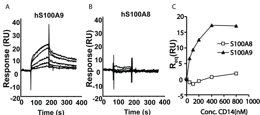
Fig 6. Interaction of CD14 with immobilized S100A8 and S100A9 using SPR analysis. Sensorgrams from bottom to top were obtained after injection of 50 to 800 nM CD14 over S100A9 (A) or S100A8 (B). Responses at steady-state ( R_{eq} ) were calculated either by fit of sensorgrams to a 1:1 model (S100A9) or at late association phase (t 175 s) due to too fast kinetics (S100A8) and plotted vs CD14 concentration in C. A K_D of 0.1 to 0.2 \mu M was calculated for CD14 binding to S100A9 whereas non-saturable binding was obtained to S100A8. The data shows representative results from one out of two experiments performed.
