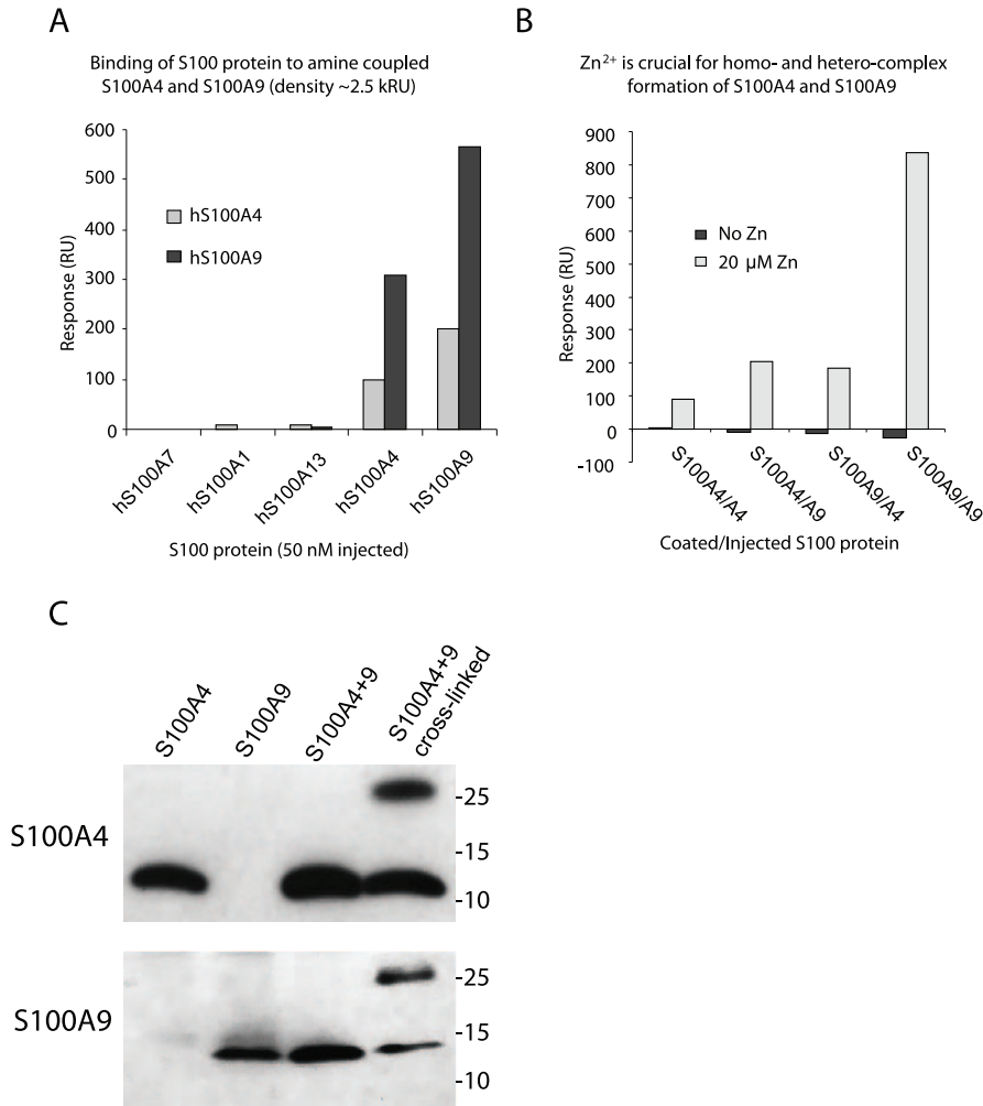
Figure 4. S100A4 and S100A9 can form heterodimers. A: Binding of S100 proteins to immobilized S100A4 and S100A9. S100A1, A4, A7, A9 and A13 (~1.3 \mu g/mL) were injected (2 min at 30 \mu L/min) over S100A4 and S100A9 (density ~2.5 kRU) in the presence of 1 mM Ca^{++} and 20 \mu M Zn^{++} . Responses were calculated at late association phase. B: Formation of homo- and hetero-complexes of S100A4 and S100A9 is Zn^{++} dependent. S100A4 and S100A9 were injected over immobilized S100A4 or S100A9 at ~1.3 \mu g/mL HBS-P containing 1 mM Ca^{++} \pm 20 \mu M Zn^{++} . Responses at late association phase were calculated. C: HEK293T cells were transfected either with S100A4 or S100A9 cDNA construct alone or the two together, as indicated. After 24 hrs of culture some of the transfected cells were exposed to the membrane permeable cross-linker DSS. Thereafter cell lysates were prepared, equal amounts (30 \mu g) of protein loaded on an SDS-PAGE gel and western blots were performed using either anti-S100A4 or anti-S100A9 antibodies as indicated. Representative results from one out of two experiments performed are shown.
