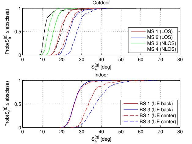
Fig. 10. Cumulative distribution of the elevation group angular spread of a group of eight users located close to each other in various outdoor (top) and indoor (bottom) scenarios. In the outdoor scenarios, plots for four UE sites, labeled MS 1–MS 4, and two BS positions, high-roof (in dashed line style) and low-roof (in solid line style) are shown. In the indoor scenarios, plots for two UE locations, back and center, and two BS positions, center (BS 1) and corner (BS 3), are shown.
