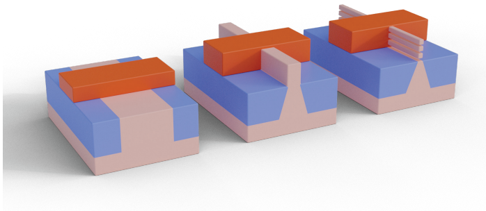
Figure 1.3 From left to right, sketches of a MOSFET, a FinFET and a GAAFET transistor. In blue is represented the body source and drain, in pink the channel and finally in orange the gate oxide.
