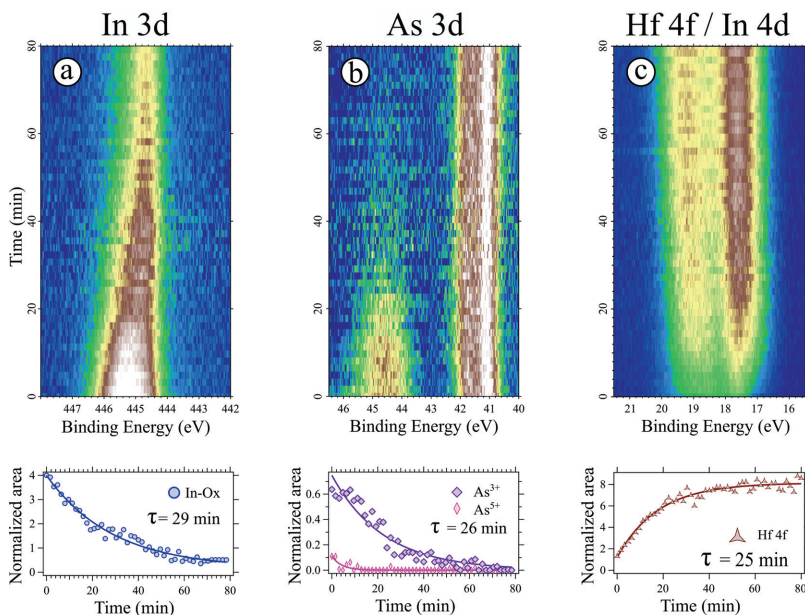
Figure 5.3 InAs oxide removal during the first half-cycle of HfO 2 ALD on InAs. From left to right (top): APXPS image plot of In 3d, As 3d and Hf 4f/In 4d core-level spectra; (bottom) Intensities evolution for In 3d oxide and As 3d oxide components and the Hf 4f line. Reprinted with permission from ref. 12. Copyright 2020 American Chemical Society.
