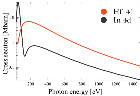
Figure 3.4 Atomic subshell photoionisation cross sections for 0-1500 eV, referred to In 4d (gray) and Hf 4f (orange). Adapted from Ref. [65].
