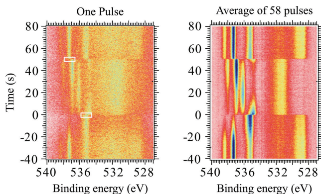
Figure 6.1 Image plots of O 1s before (left) and after (right) event-averaging. The white boxes on the left image plot are the events used to characterise the periodicity of the transitions. Adapted from ref. [47].
