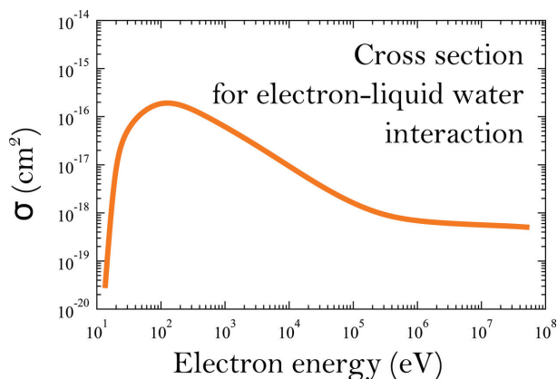
Figure 4.9 Total electron ionisation cross section for electron – water interaction. Adapted from ref.[87].
