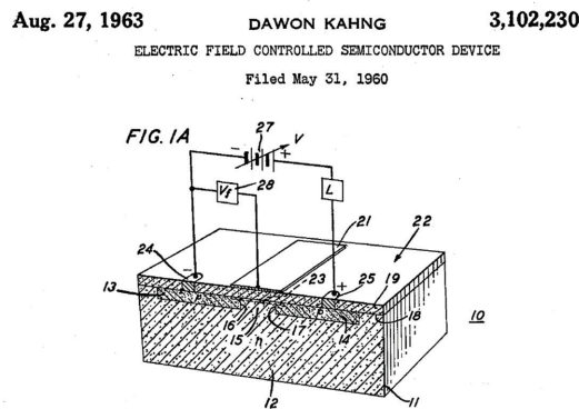
Figure 1.2 Figure from the Dawon Kahng's U.S. patent office. Source: United States Patent and Trademark Office, www.uspto.gov , ref [4]
