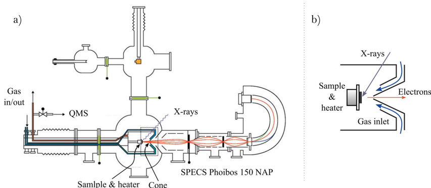
Figure 4.7 a) Schematic layout of the APXPS enedation at SPECIES, showing all the chambers. In orange, the path of the photoelectrons towards the analyser. b) Schematic view of the SPECIES cell with the double-cone system for gas inlet. Adapted from ref.[80].
