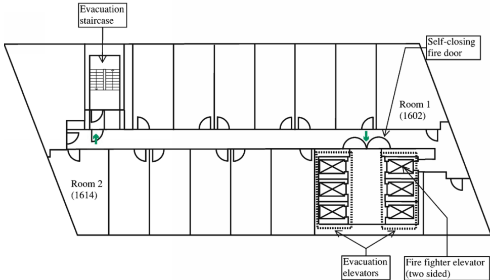
Figure 5. Floor plan of the hotel floor. The two marked rooms (Room 1 and 2) were the ones used in the experiment. The green arrows indicate the location of the evacuation signs.
