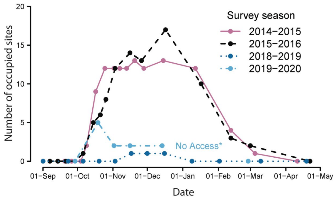
Figure 4. Seasonal changes in site occupancy of aestivating Bogong moths close to the summit of Mount Gingera in the Brindabella Ranges (on the NSW and ACT border), based on 37 sites surveyed by Caley & Welvaert (2018) during 2014–2016 (reproduced with permission), and during the recent extreme drought.
