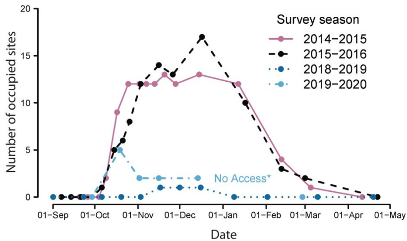
Figure 4. Seasonal changes in site occupancy of aestivating Bogong moths close to the summit of Mount Gingera in the Brindabella Ranges ( on the NSW and ACT border ), based on 37 sites surveyed by Caley & Welvaert (2018) during 2014–2016 (reproduced with permission), and during the recent extreme drought.
