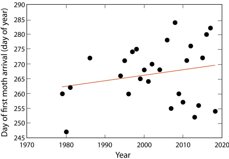
Figure 3. Date of first arrival of the Bogong moths above the snowline in the Snowy Mountains from 1979 until the present. Regression line has the following equation: D = 0.19Y - 114 ( R^2 = 0.050 ) where D is the day of the year for the first moth arrival, and Y is the year.
