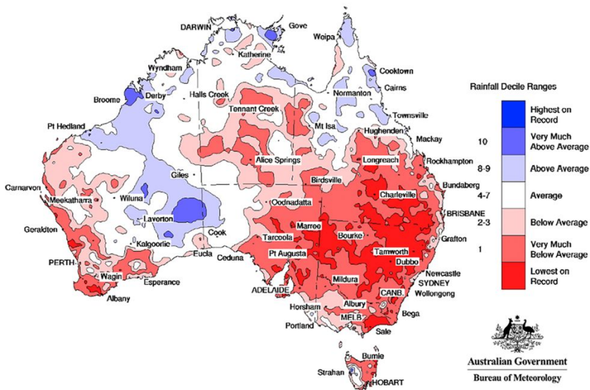
30 31 32 33 34 35 36 37 38 39 40 41 42 43 44 45 46 47 48 49 50 51 52 53 54 55 56 57 58 59 60 Figure 5. Australian rainfall deciles (1 January 2017 – 31 December 2019). Source: Bureau of Meteorology, Australian Government. Distribution based on gridded data.
