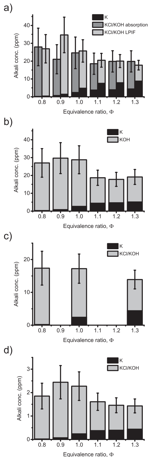
Fig. 7. Bar charts illustrating balance of alkali species concentrations for the investigated flames. The sum of K-atom concentrations (black bars) and KCl/KOH concentrations (grey bars) is constant within the experimental uncertainties indicated by the error bars. (a) 1.0 M KCl seeding, (b) 0.5 M KOH seeding, (c) 0.5 M KCl seeding, and (d) 0.05 M KCl seeding. KCl/KOH concentration measured by laser-induced photofragmentation fluorescence are presented with light grey bars for all the flames. For the 1.0 M flame presented in (a), KCl/KOH concentrations were also measured by absorption spectroscopy and these values are presented with dark grey bars.
