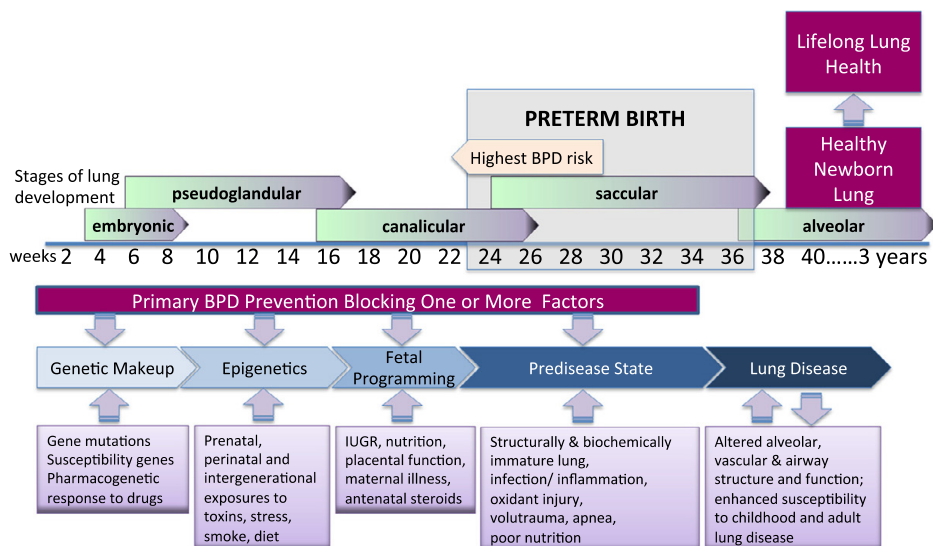
Figure 2. Etiology of bronchopulmonary dysplasia.
