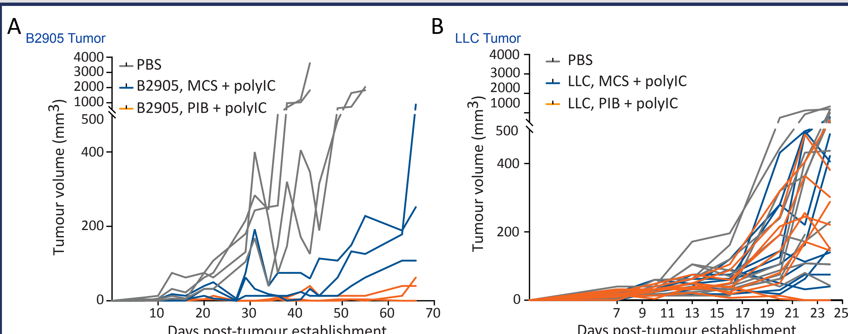
Fig 5. Anti-Tumor Immune Response Elicited by Tumor-APCs Correlates with Cross-Presentation Capacity. WT tumors were established and injected with polyI:C stimulated tumor cells transduced with PIB or MCS or injected with PBS at day 10 post-tumour establishment. A) Tumor growth in mice injected with B2905 tumor cells and tumor-APCs or empty vector (MCS) control transduced cells or PBS (n=3-4). B) Tumor growth in mice injected with LLC tumor cells and tumor-APCs or empty vector (MCS) control transduced cells or PBS (n=10).
