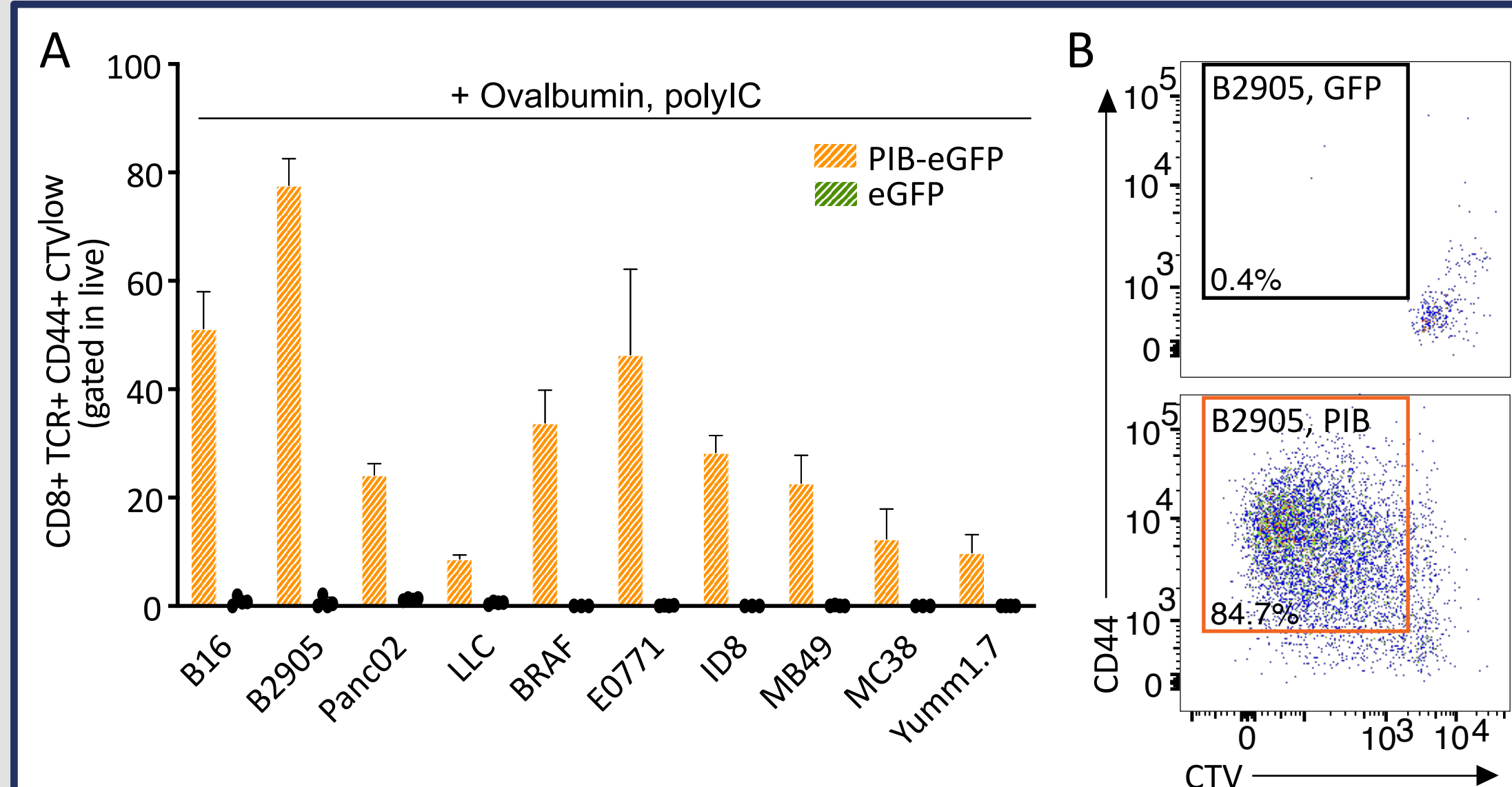
Fig 2. PU.1, IRF8 and BATF3 Endow Mouse Cancer Cells with cDC1 Function Cross-Presentation. Tumour-APCs at reprogramming day 8 were pulsed with ovalbumin antigen and polyI:C before co-culture with ovalbumin-specific naive CD8+ T cells (OT-I) for 3 days. OT-I cells were membrane-labelled with CellTrace violet (CTV) to measure proliferation and stained for activation marker CD44. A) Quantification of CD44+ proliferative OT-I CD8+ T cells after co-culture. (n=4) B) Representative flow cytometry plot of CD8+ T cell proliferation (CTV) and activation (CD44) after co-culture with PIB-eGFP transduced (lower) and control eGFP transduced (upper) B2905 cells.
