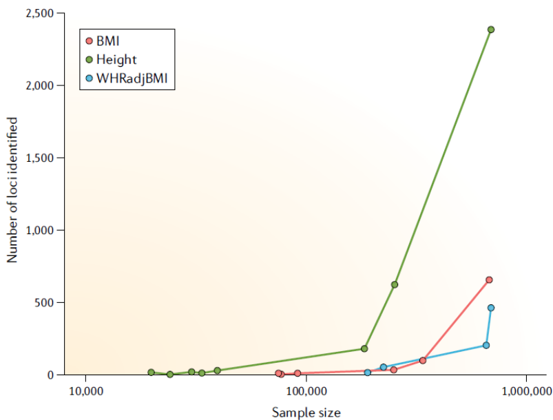
Figure 5: Number of loci identified as a function of GWAS sample size. Number of genome- wide significant loci reported from GWAS for three anthropometric traits: body mass index, height and waist-to-hip ratio adjusted for BMI. Reprint with permission from Tam et al. , 2019.
