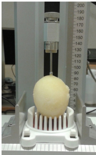
Figure 7. Texture analysis of a whole potato tuber by puncture with a spherical probe. The picture was taken by the author.
