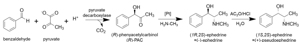
Fig. 3.5 Carbolication of pyruvate and benzaldehyde producing ( R )-phenylacetylcarbinol, which can then be transaminated to (1 R ,2 S )-(-)-ephedrine. Adapted from [121]
