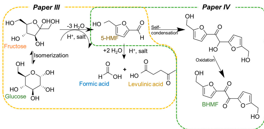
Fig. 5.1. Overview of the valorisation work from glucose/fructose to levulinic acid via 5-HMF pathway ( Paper III ) and carboligation of 5-HMF into C 12 compounds 5,5'-bis(hydroxymethyl) furon (DHMF) and 5,5'-bis(hydroxymethyl)fural (BHMf) ( Paper IV )
