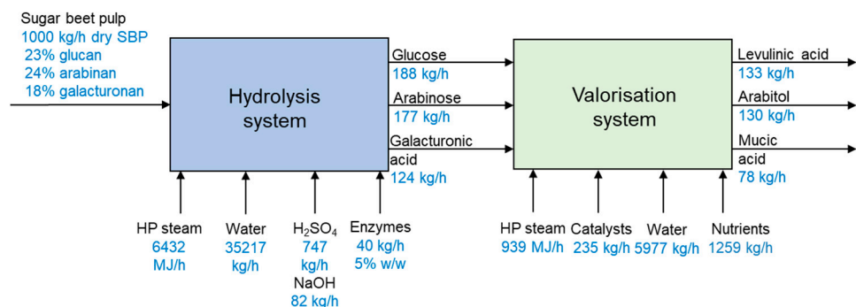
Fig. 6.4. Mass and energy flows for the hydrolysis and valorisation system in the proposed sugar beet pulp-based biorefinery with an input capacity of 1000 kg/h dry SBP. Adapted from Paper I .
