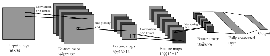
Figure 10: An example of a CNN architecture. In this figure the layers with the activation function are included in the convolutional layers.
