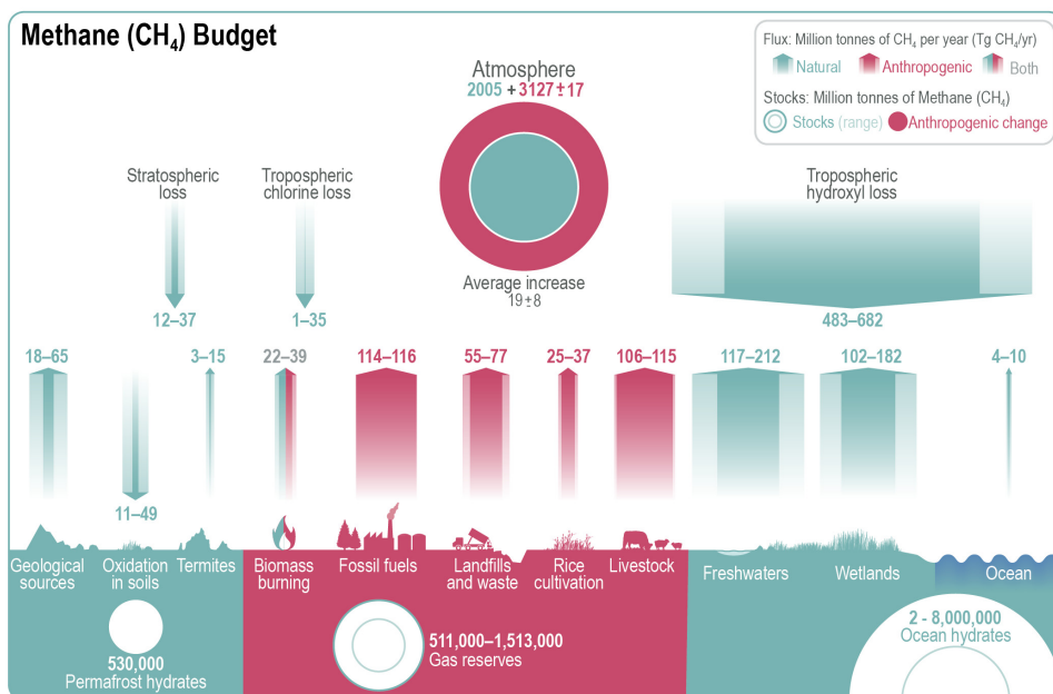
Figure 1: Global methane (CH 4 ) budget (2008–2017). The atmospheric stock is calculated from mean CH 4 concentration, multiplying a factor of 2.75 \pm 0.015 Tg ppb -1 , which accounts for the uncertainties in global mean CH 4 (adapted from Chandra et al., 2021).
